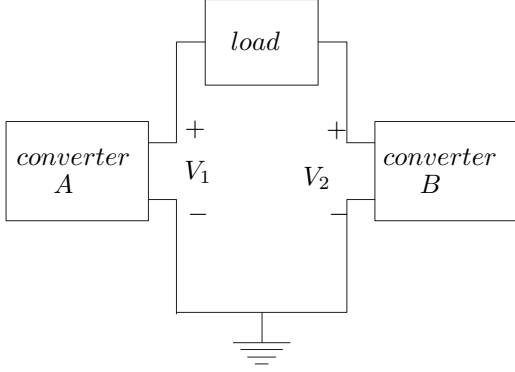
Fig. 1. Basic representation of the boost inverter.
