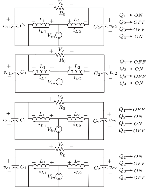
Fig. 3. Operation modes
