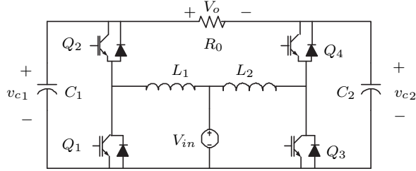
Fig. 2. Ideal Boost DC-AC Converter.
