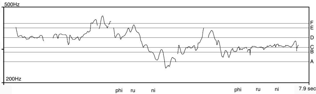
Fig. 7 Melodic transcription of the bottom line in fig. 6
