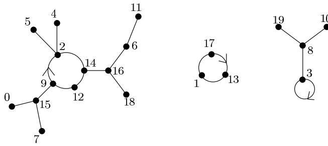
FIG. 4. a unary function f_0 over D = \{0, \dots, 19\}
