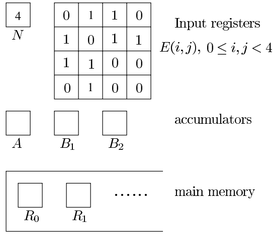
FIG. 1. an NRAM for a graph problem
