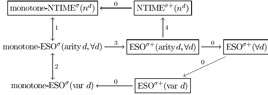
FIG. 2. Inclusions between the complexity classes
