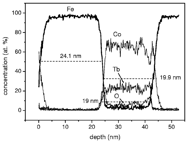
FIG. 4. Concentration depth profiles obtained perpendicular to the TbCo 2.5 /Fe film planes.
