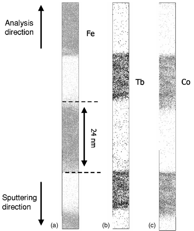
FIG. 3. Three-dimensional reconstruction of a given analyzed volume in a TbCo 2.5 /Fe multilayer with different depicted atoms: (a) Fe; (b) Tb (including Tb oxides and hydrides); and (c) Co atoms. The volume was reoriented along the normal to interfaces.
