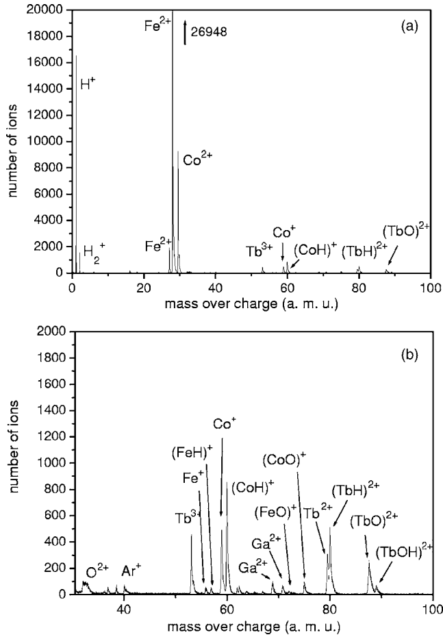
FIG. 2. Mass spectra related to the analysis of TbCo 2.5 /Fe multilayers using the tomographicatom probe (a). Inset is the magnification in the 30–100 mass over charge range (b).
