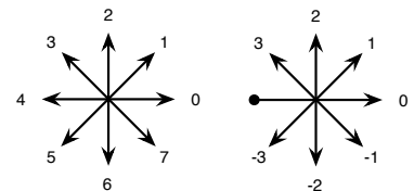
(a) Freeman codes (b) Differential Freeman codes
