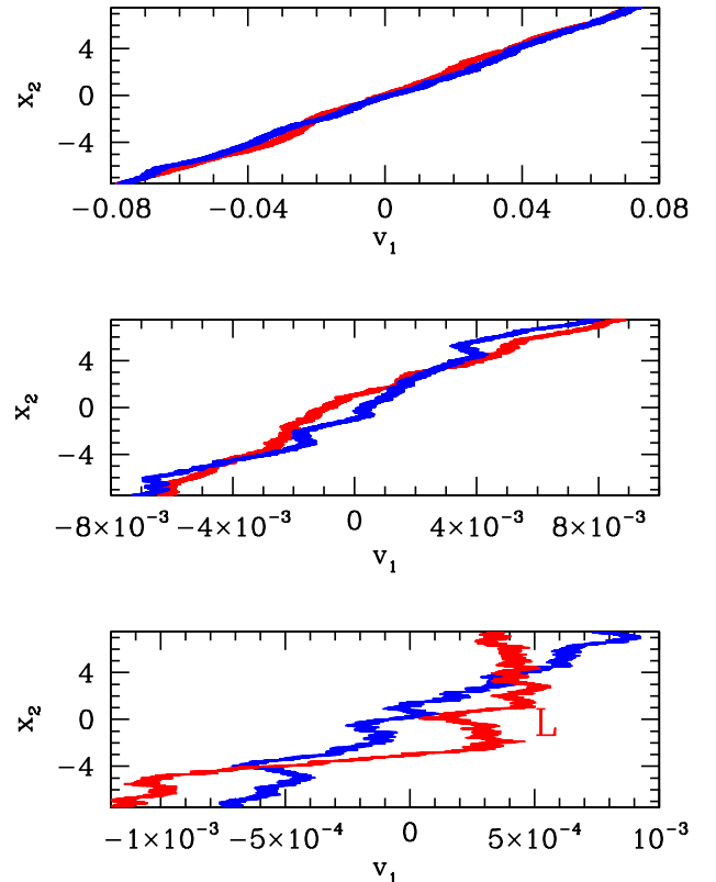
FIG. 3: (Color online) Two velocity profiles at randomly chosen times, for I = 3.2 \times 10^{-2} (top), I = 3.2 \times 10^{-3} (middle), I = 3.2 \times 10^{-4} (bottom). \kappa = \kappa_1 , \zeta = 0.98 and N = 4000 .
