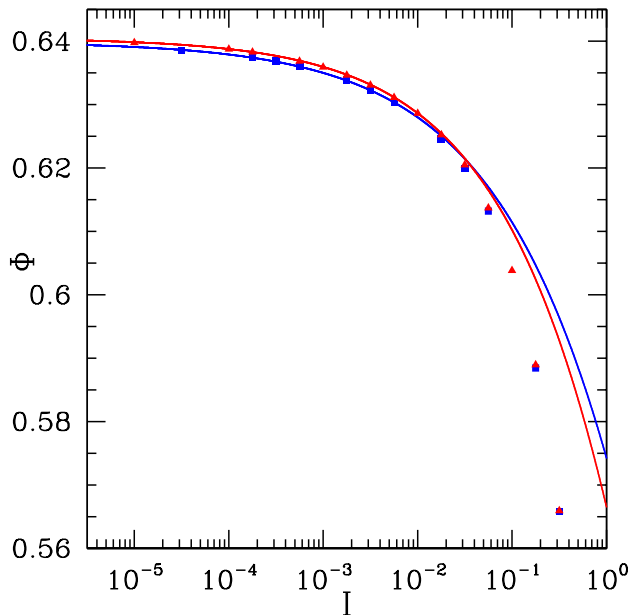
FIG. 7: (Color online) Volume fraction \Phi as a function of inertial number I (for \zeta = 0.98 , N = 4000 ), for both stiffness levels \kappa = \kappa_1 (blue squares) and \kappa = \kappa_2 (red triangles). The solid lines are given by Eq. (11) with the parameters of Table V.
