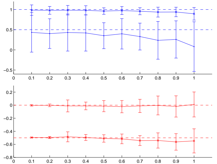
Fig. 2. Average performance of the automatic tuning with respect to the noise level over 100 runs. Expectation of the estimated parameters a_1, b_1 (top) and a_2, b_2 (bottom) with their standard deviations versus the noise level \beta_2 . The true parameters are also represented (dash lines).
