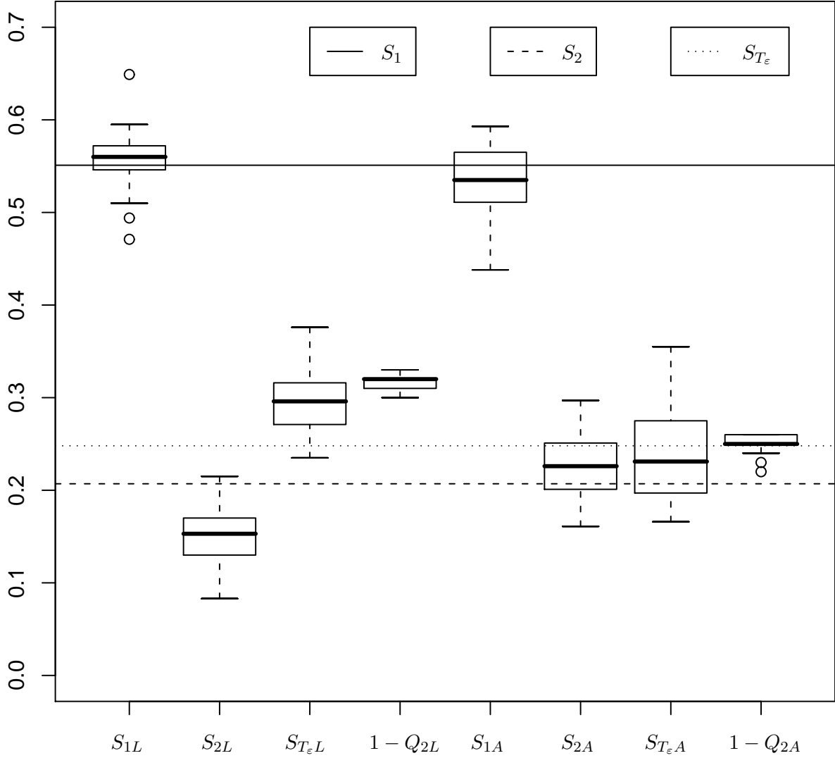
Figure 1: WN-Ishigami application. Comparison of Sobol indices estimates. Reference values: S_1, S_2, S_{T_\epsilon} . Joint GLM: S_{1L}, S_{2L}, S_{T_\epsilon L}, 1 - Q_{2L} . Joint GAM: S_{1A}, S_{2A}, S_{T_\epsilon A}, 1 - Q_{2A} . 1 - Q_{2L} (resp. 1 - Q_{2A} ) is the estimation of S_{T_\epsilon} via the joint GLM (resp. joint GAM) Q_2 coefficient. Learning sample size: n = 200 .
