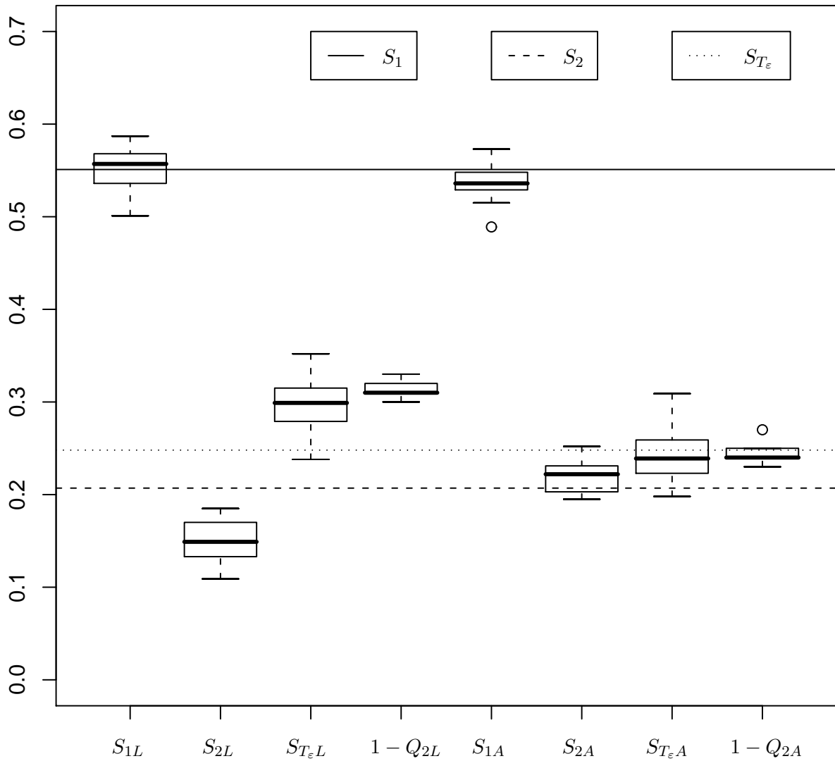
Figure 2: WN-Ishigami application. Comparison of Sobol indices estimates. Reference values: S_1, S_2, S_{T_\epsilon} . Joint GLM: S_{1L}, S_{2L}, S_{T_\epsilon L}, 1 - Q_{2L} . Joint GAM: S_{1A}, S_{2A}, S_{T_\epsilon A}, 1 - Q_{2A} . 1 - Q_{2L} (resp. 1 - Q_{2A} ) is the estimation of S_{T_\epsilon} via the joint GLM (resp. joint GAM) Q_2 coefficient. Learning sample size: n = 500 .
