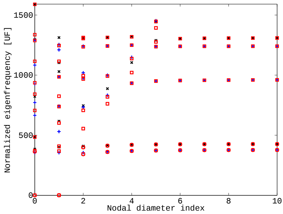
Figure 8. Influence of interstage coupling, Eigenfrequency/nodal diameter map (from 0 to 10 ND), stage 1 alone \times , stage 2 alone + , coupled stages \square .
