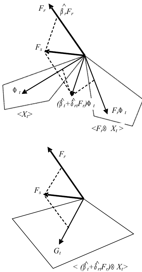
Figure 11: Internal estimation of an interactive variable
