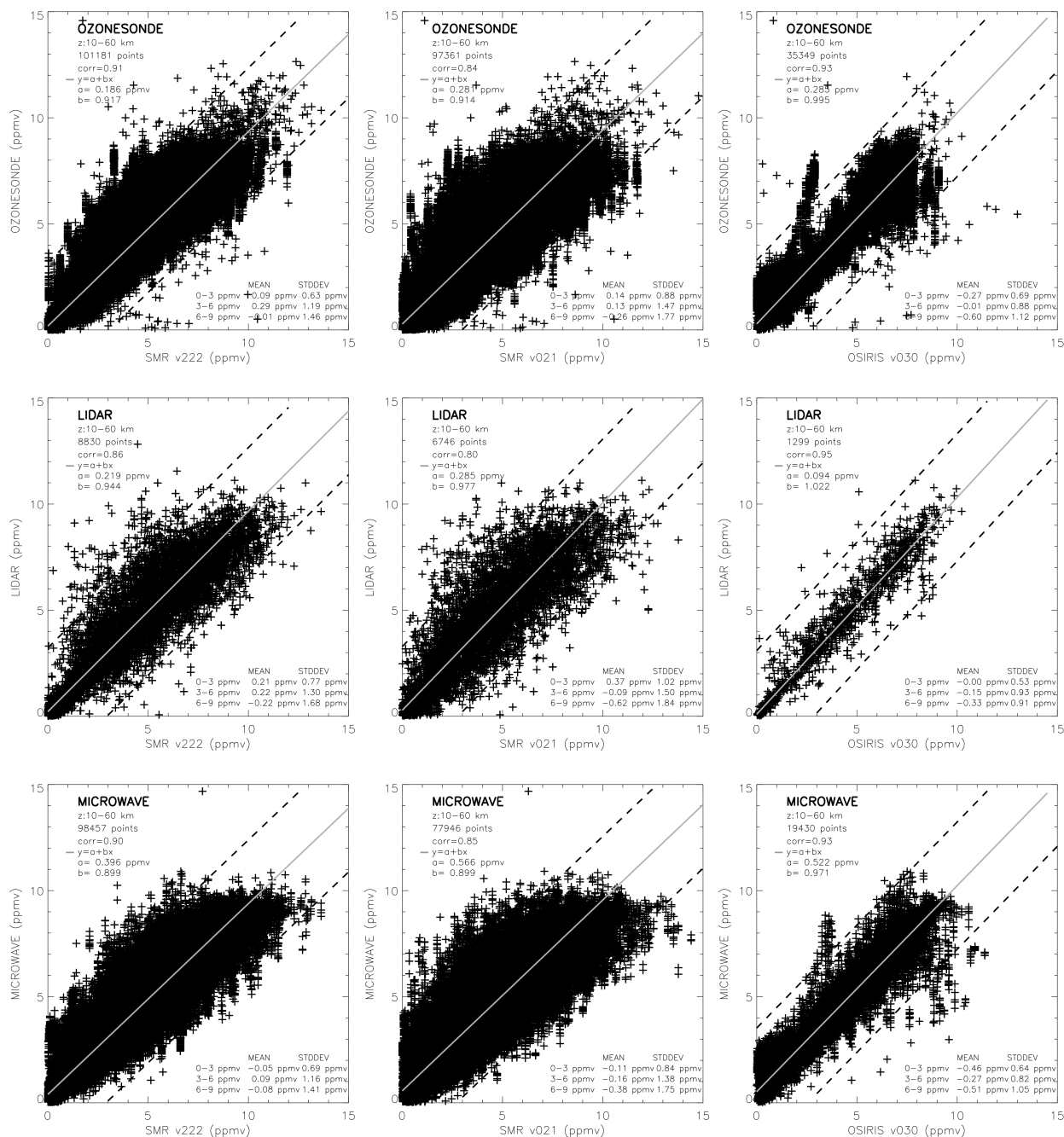
Fig. 9. Scatterplot of Odin/SMR and OSIRIS O 3 versus NDACC measurements. Left: Odin/SMR v222 data; middle: Odin/SMR v2.1 data; right: Odin/OSIRIS v3.0 data. Top: Ozone sonde, Middle: Lidar, Bottom: Micro-wave. Mean differences and standard deviations are indicated for the different ranges of the O 3 mixing ratio. The dotted lines delimit deviations of \pm 3 ppmv for clarity. The solid gray line indicates the linear fit to the data.
