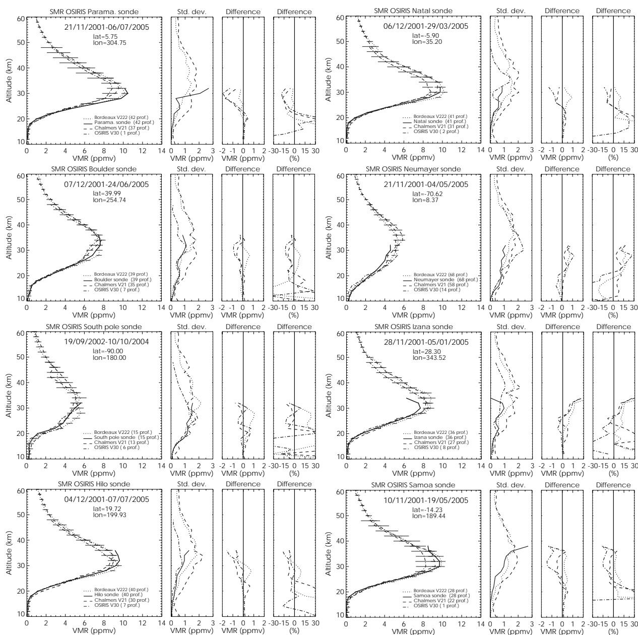
Fig. 7. Same as Fig. 3 but for monthly mean OSIRIS, SMR and ozone sonde profiles for eight NDACC stations: Paramaribo, Natal, Boulder, Neumeyer, South Pole, Izana, Hilo and Samoa Islands.
