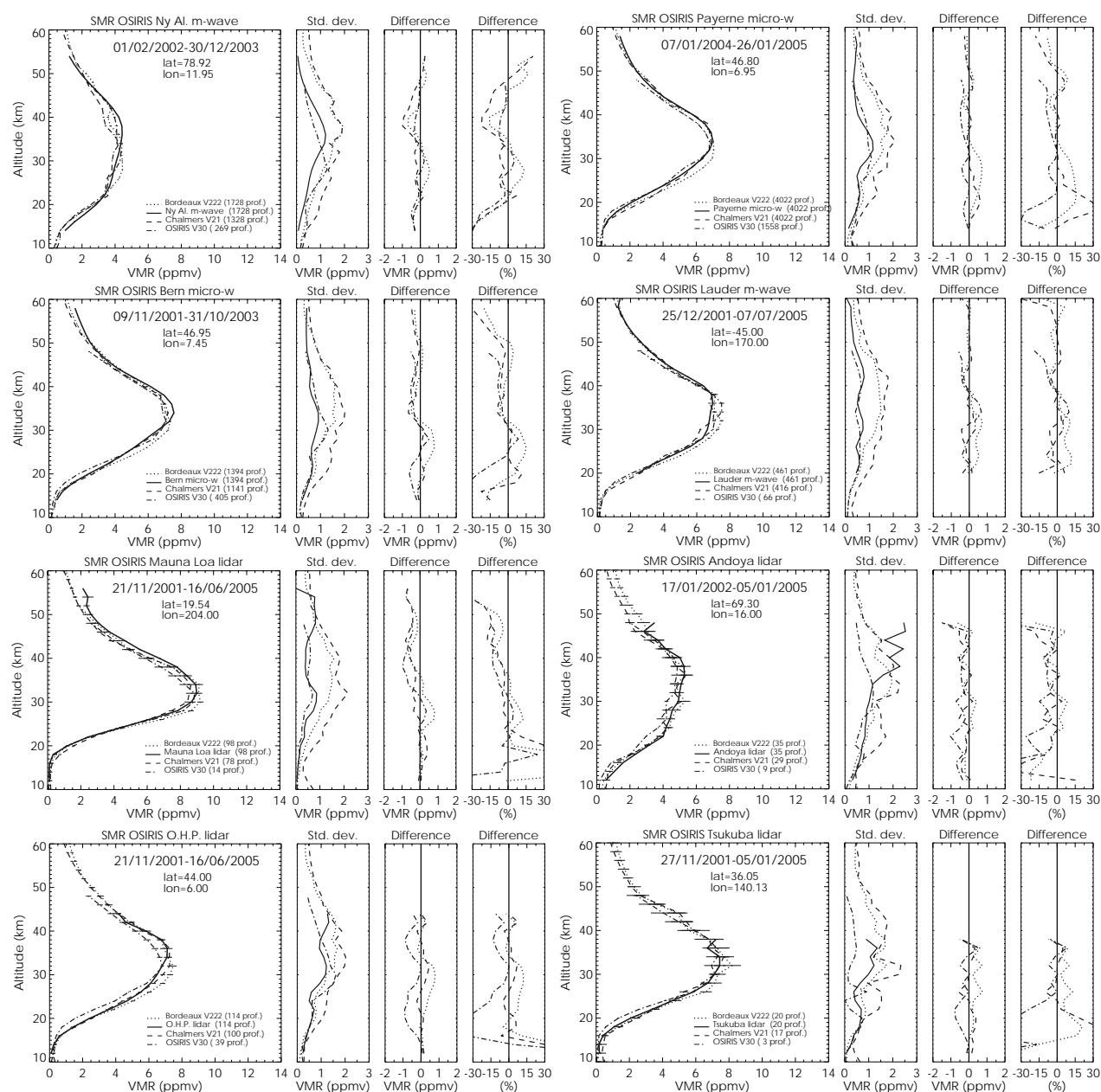
Fig. 8. Same as Fig. 7 but for comparisons of monthly mean OSIRIS, SMR and NDACC profiles performed in four microwave (Ny Alesund, Payerne, Bern, Lauder) and four lidar NAADC stations (OHP, Tsukuba, Mauna Loa, Andoya).
