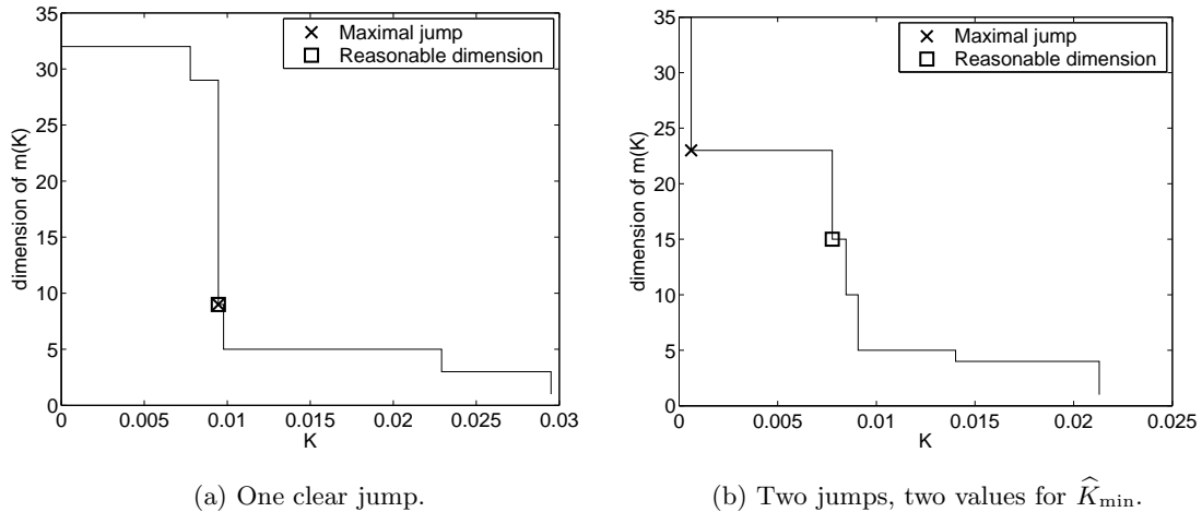
FIG 1. D_{m(K)} as a function of K for two different samples. Data are simulated with X \sim \mathcal{U}([0, 1]) , \epsilon \sim \mathcal{N}(0, 1) , s(x) = \sin(\pi x) , \sigma \equiv 1 , n = 200 . (S_m)_{m \in \mathcal{M}_n} is the collection of regular histogram models with dimension between 1 and n/(\ln(n)) . \text{pen}_{\text{shape}}(m) = D_m . “Reasonable dimensions” are below n/(2 \ln(n)) \approx 19 . See Sect. 5.4 in [Arl07] for details (experiment (S1)).
