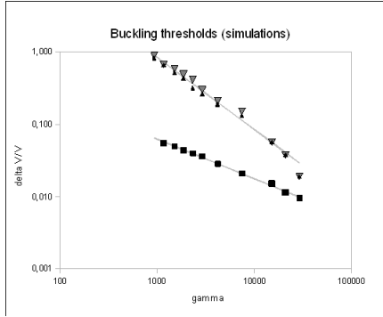
Figure 10: Primary buckling (black squares) from sphere to capsule: relative volume at which the axisymmetric depression appears in the simulations, for different \gamma . Interpolating straight line : \frac{\Delta V}{V} = 2.8 \gamma^{-0.55} . Secondary buckling: polygonization of the circular rim (black upwards pointing triangles) and apparition of wrinkles (gray downwards pointing triangles). Interpolating straight line: \frac{\Delta V}{V} = 850 \gamma^{-1} .
