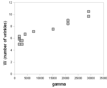
Figure 5: Number W of wrinkles hold by the single depression after secondary buckling, averaged between \frac{\Delta V}{V} = 0.53 and \frac{\Delta V}{V} = 0.76 , as a function of the dimensionless Föppl-von Karman number \gamma = \frac{AR^2}{\kappa} .
