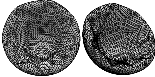
Figure 11: Simulation with \gamma=15163 , \nu=0.333 and \frac{\Delta V}{V}=0.645 . Such unusual conformation can be obtained from a capsule at lower \gamma ; its energy is 1.42 times lower than the configuration with wrinkles ( W=7 ) obtained through progressive volume decrease for similar parameters.
