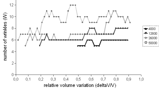
Figure 4: Typical evolution of the number W of wrinkles hold by the single depression after secondary buckling (simulations performed for 4 values of \gamma , \nu=0.333 ).
