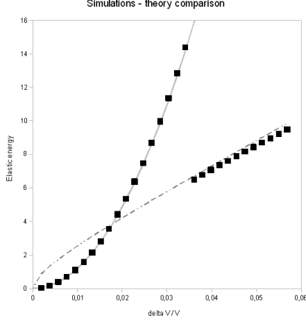
Figure 9: Elastic energy of a shrinking shell. Black squares: result of Surface Evolver simulations, with \gamma=2916 (volume of the initial sphere: V_0=5.268 ( R=1.08 ), \kappa=2 , A=5000 ) and \nu=0.333 . Continuous line: elastic energy of a shrinking spherical shell, according to equation 4 with same parameters. Interrupted line: elastic energy of a capsule (deformation with a single axisymmetric depression) according to equations 5 and 6, with same parameters.
