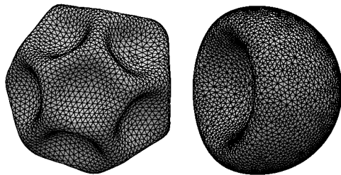
Figure 3: Conformations numerically obtained with Surface Evolver for \gamma=743 , \nu=0.333 (which corresponds to a shell of relative thickness d/R=0,116 of an incompressible material with \sigma=0,5 ), \frac{\Delta V}{V}=0.171 , c_0 = 1/R , 3594 vertices. Left: simulation performed by directly minimizing at c_0 = 1/R for each decreasing volume step: N=17 depressions. Right : simulation performed first with c_0 = 0 , then c_0 = 1/R . The elastic energy is 3.10 times larger for the “potato” (left) than for the capsule (right).
