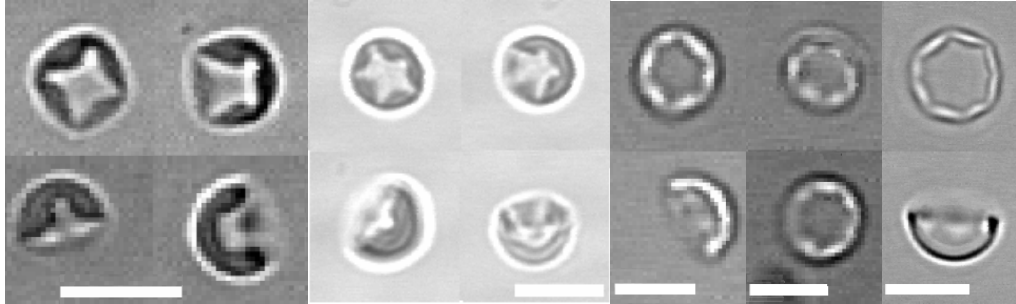
Figure 2: Spherical shells buckled in solution, showing 4 to 8 wrinkles (a-e). Each sub-figure shows different transmission optical microscopy views of the same object. Scale bar 5\mu m , except subfigure c: 2\mu m .
