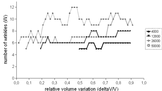
Figure 4: Typical evolution of the number W of wrinkles hold by the single depression after secondary buckling (simulations performed for 4 values of \gamma , \nu=0.333 ).
