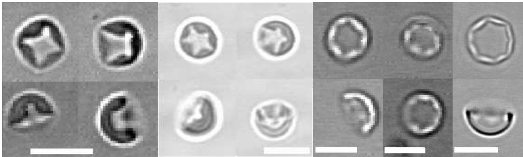
Figure 2: Spherical shells buckled in solution, showing 4 to 8 wrinkles (a-e). Each sub-figure shows different transmission optical microscopy views of the same object. Scale bar 5\ \mu\text{m} , except subfigure c: 2\ \mu\text{m} .
