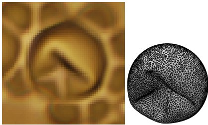
Figure 8: (a) Shell enclosing oil, evaporated in air ( d/R \approx 0.012 ). Transmission optical microscopy, size 17 \mu\text{m} \times \mu\text{m} . (b) Simulation obtained for \gamma=2916 and \nu=0.333 (equivalent to \frac{d}{R}=0.064 ), by increasing the volume from \frac{\Delta V}{V}=0.474 to \frac{\Delta V}{V}=0.209 , 3659 vertices.
