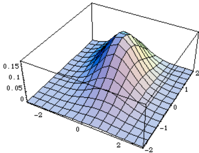
Figure 2 The bivariate normal density function for 1998
