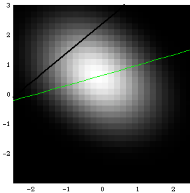
Figure 5 Party partition, 1998 average PUNEs, \beta=1.4
