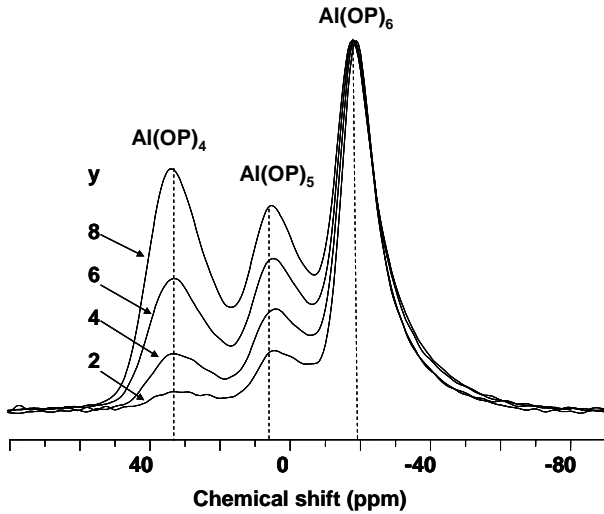
Figure 6. ^{27}\text{Al} MAS NMR spectra of ZnPbCdPAL glasses
