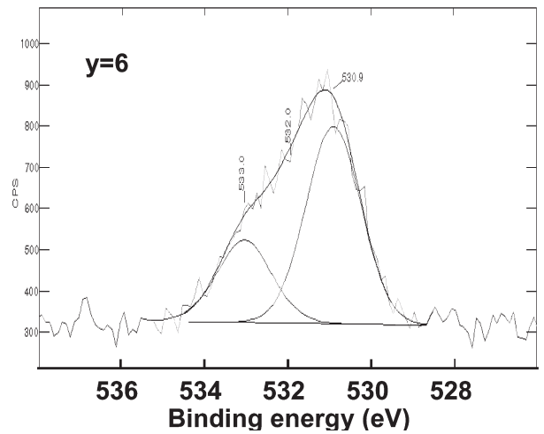
Figure 7. Examples of decomposition of XPS O1s spectra of x=20 ZnPbCdP glass and y=6 ZnPbCdPAL glass
