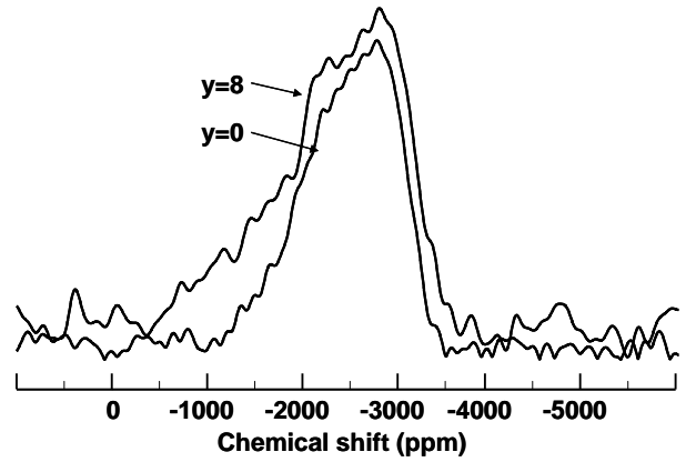
Figure 5. ^{207}\text{Pb} MAS NMR spectra of y=0 and 8 ZnPbCdPAL glasses
