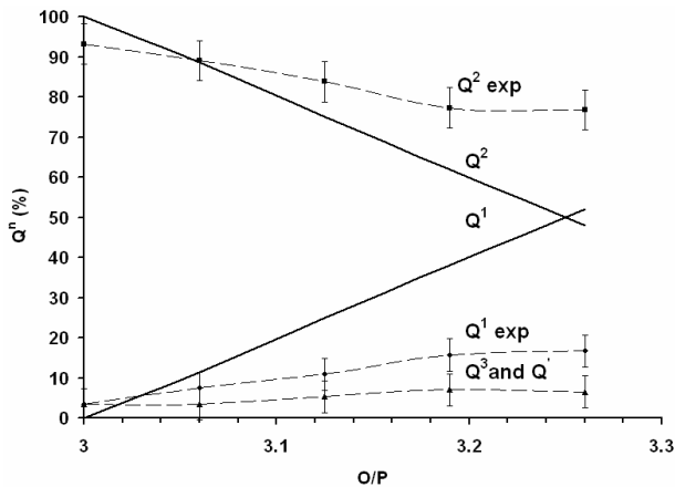
Figure 8. Fractions of Q^n sites deduced from the decomposition of ^{31}\text{P} MAS NMR spectrum (dashed line), compared to those calculated (continuous line) assuming a complete dissolution of \text{Al}_2\text{O}_3 in the \text{ZnPbCdP} melt
