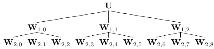
Fig. 2. 3-DWPT decomposition tree of \mathbf{U} down to resolution level j = 2 .
