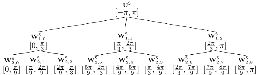
Fig. 4. Re-ordering of the Shannon 3-DWPT decomposition tree. The positive part of the support of \mathcal{F}W_{j,n}^S is indicated below \mathbf{W}_{j,n}^S .
