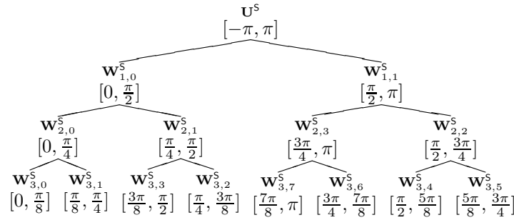
Fig. 3. Re-ordering of the Shannon 2-DWPT decomposition tree. The positive part of the support of \mathcal{F}W_{j,n}^S is indicated below \mathbf{W}_{j,n}^S .
