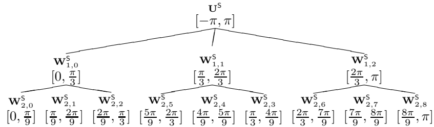
Fig. 4. Re-ordering of the Shannon 3-DWPT decomposition tree. The positive part of the support of \mathcal{F}W_{j,n}^S is indicated below \mathbf{W}_{j,n}^S .
