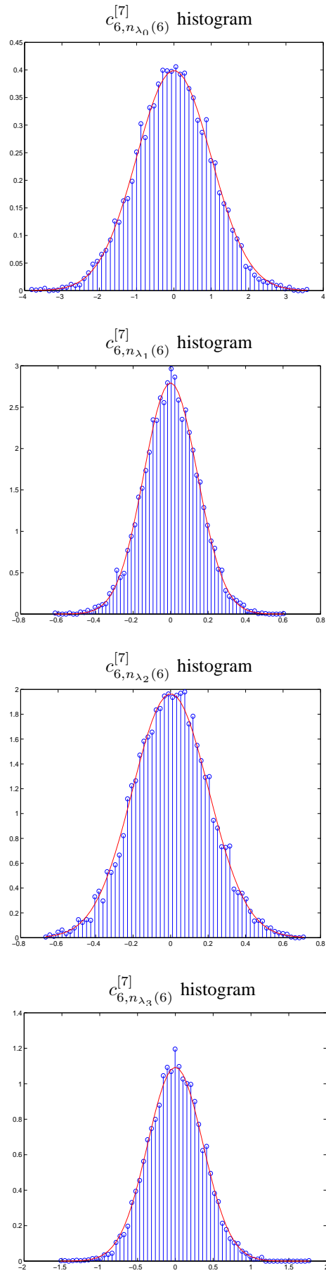
Fig. 7. Histograms of the DWPT coefficients, at resolution level 6, using Daubechies filters of order 7. The decomposition is applied to samples of an AR(1)-GG process with \alpha given by Eq. (58), \beta = 1 and \mu = 0.75 . The limit distribution \mathcal{N}(0, \gamma(a(\lambda))) where a(\lambda_0) = 0 and a(\lambda_q) = \pi/2^{q-1} for q = 1, 2 and 3 is represented by the (red) continuous line.
