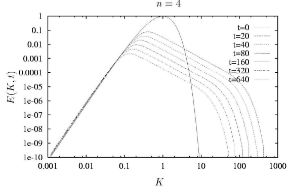
Figure 1: Turbulent kinetic energy spectrum for isotropic turbulence. EDQNM model. Results plotted at different times.
