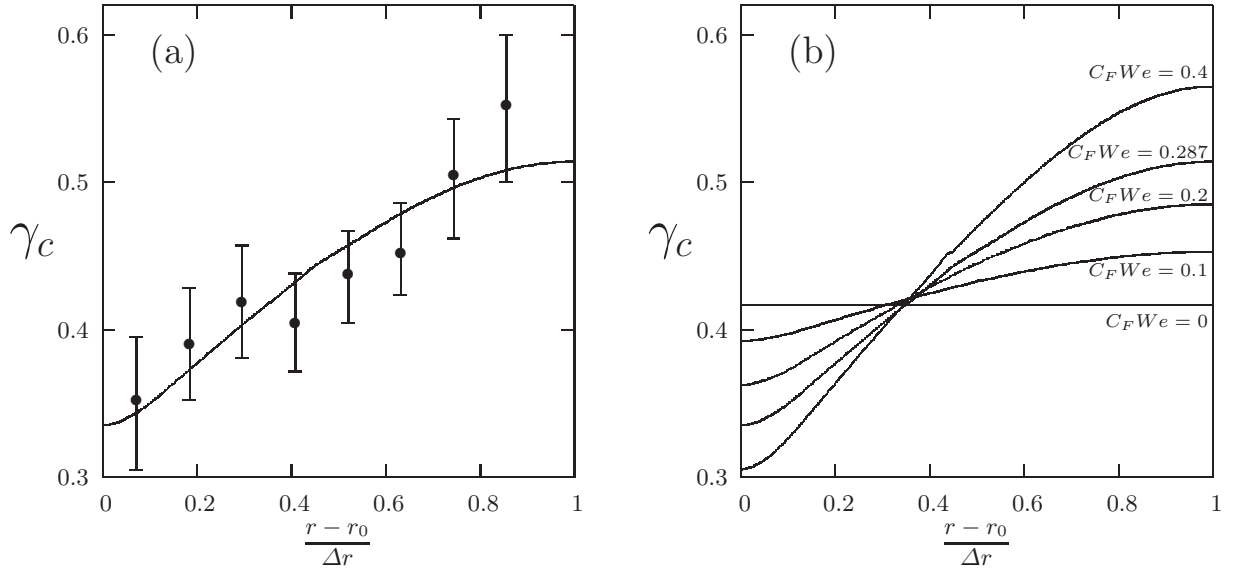
Fig. 5. Transient case: (a) \gamma_c versus r with parameters as in table (1). \bullet : experimental data with error bars; solid line: numerical data. (b) \gamma_c versus r with Bi and We as in table (1) and C_F We = 0, 0.1, 0.2, 0.287, 0.4 .
