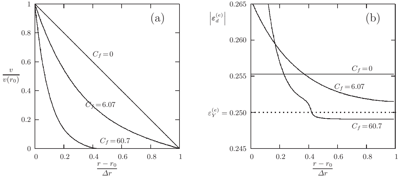
Fig. 12. Stationary plane Couette case with Bi = 85 , We = 5.88 \times 10^{-3} and C_F varying: (a) velocity profile ; (b) |\epsilon_d^{(e)}| .
