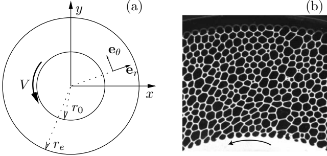
Fig. 1. Experimental set-up: (a) definition of the geometric and kinematic parameters ; (b) picture of the confined bidimensional liquid foam (from [1]).
