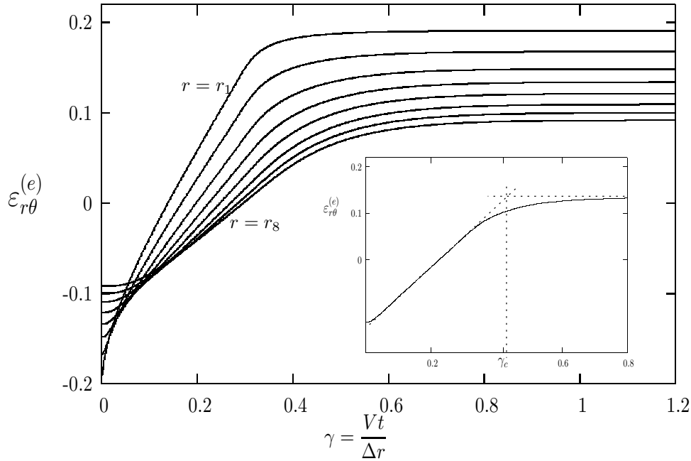
Fig. 4. Transient case: cross component of the elastic strain \varepsilon_{r\theta}^{(e)} versus t for r = r_1 to r_8 . Inset: the vertical dashed line mark the cross-over \gamma_c between the transient and the stationary regimes, defined by the intersection of the tangent at the point of minimum curvature and the asymptotic value of \varepsilon_{r\theta}^{(e)} , here plotted for r = r_4 .
