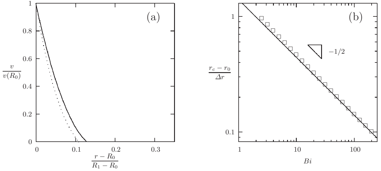
Fig. 11. Stationary case: (a) velocity profile for Bi = 85 , We = 5.88 \times 10^{-3} ; C_F = 0 (solid line) or C_F = 60.7 (dashed line). (b) Localisation point versus Bi for the stationary Bingham fluid ( We = C_F = 0 ); \square : exact analytical result (10); solid line: approximate numerical prediction (11).
