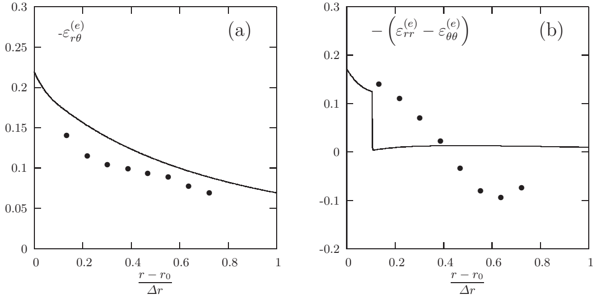
Fig. 9. Stationary case: Solid line: numerical resolution; \bullet : experimental data from [12]. (a) Shear component -\epsilon_{r\theta}^{(e)} versus r . (b) Difference of normal components -(\epsilon_{rr}^{(e)} - \epsilon_{\theta\theta}^{(e)}) versus r .
