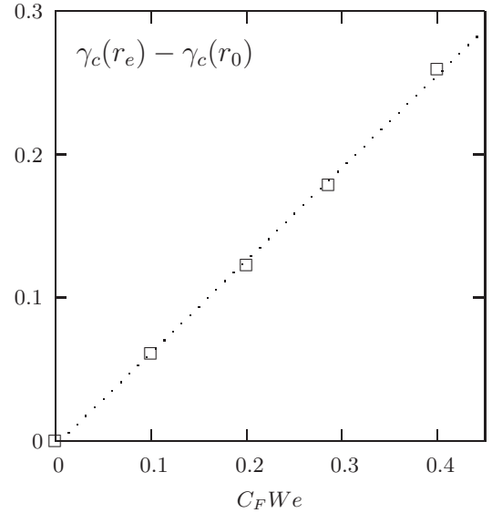
Fig. 6. Transient case: \gamma_c(r_e) - \gamma_c(r_0) versus C_F We . \square : numerical data; dashed line: linear fit to these data.
