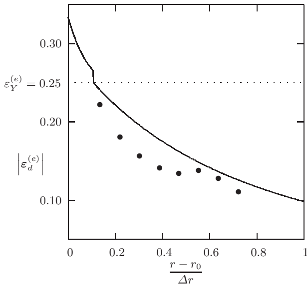
Fig. 10. Stationary case: |\varepsilon_d^{(e)}| versus r . Solid line: numerical resolution; \bullet : experimental data from [12].
