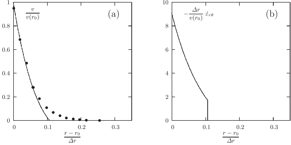
Fig. 8. Stationary case: (a) Velocity versus r . Solid line: computation; \bullet : experimental data from [1]. (b) Shear strain rate \dot{\epsilon}_{r\theta} versus r . There is no experimental data available for the comparison.
