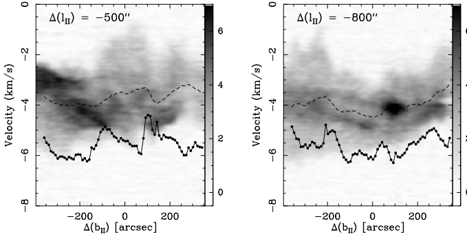
Fig. 10. Position-velocity cuts at constant \ell_{II} offsets ( \Delta\ell_{II} = -500'' , left and \Delta\ell_{II} = -800'' , right). Grey-scale: main-beam intensity in K. Dashed curve: centroid velocity. Full curve: azimuthally averaged CVI for a lag l = 3 pixels (with an additional offset of -6.5 \text{ km s}^{-1} for clarity).
