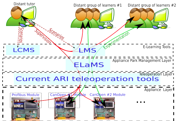
Figure 10. Final platform architecture
