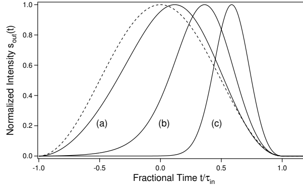
Figure 3: Intensity profile of the output pulses obtained in the case of an input pulse without background for A_{in} = (a) 1, (b) 10 and (c) 100 with \tau/\tau_{in} = (a) 0.6 (b) 1.5 and (c) 4.2 (the value maximizing the fractional delay in each case). The profile of the input pulse (cos-pulse) is given for reference (dashed line).
