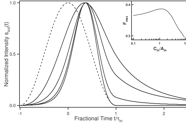
Figure 6: Intensity profile of the output pulses obtained for an overall peak intensity A_{in} + C_{in} = 10 . In order of increasing width, the represented profiles correspond to C_{in}/A_{in} = 0, 0.11, 0.54 and 9.0 . For each value of C_{in}/A_{in} , \tau/\tau_{in} is optimized in order to maximize the fractional delay. The profile of the input pulse (cos-pulse) is given for reference (dashed line). Inset: F_{max} as a function of C_{in}/A_{in} .
