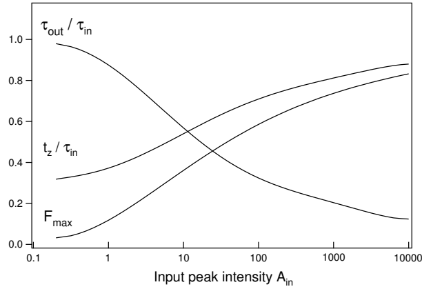
Figure 4: F_{max} , t_Z/\tau_{in} and \tau_{out}/\tau_{in} as functions of the peak intensity A_{in} in the case of cos-pulses. For A_{in} \geq 1000 , the ratio \tau/\tau_{in} maximizing F and F_{max} itself are well approximated by the asymptotic formula \tau/\tau_{in} \approx (2A_{in}^2/\pi^2)^{1/5} and F_{max} \approx 1 - (128/\pi^4 A_{in})^{1/5} .
