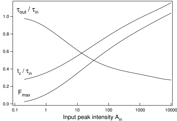
Figure 5: Same as Fig. 4 in the case of gaussian pulses. The ratio \tau/\tau_{in} maximizing F is 0.6, 1.5, 5.0, 14 and 42 respectively for A_{in} = 1, 10, 100, 1000 and 10000 .
