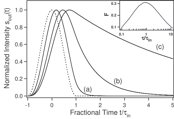
Figure 2: Intensity profile of the output pulses obtained in the case of small modulation index for \tau/\tau_{in} = (a) 0.2 (b) 0.9 and (c) 5. The profile of the input pulse (cos-pulse) is given for reference (dashed line). The time unit is its full width at half maximum \tau_{in} . Inset: Fractional delay as a function of the ratio \tau/\tau_{in} .
