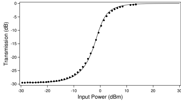
Figure 1: Transmission at 1530 nm of a erbium-doped optical fiber as a function of the incident power. The parameters are L = 7.5 m and \alpha L = 6.8 . The points are experimental [30] and the continuous line is obtained from Eq. 5 by adjusting the saturation power P_{sat} . The best fit is obtained for P_{sat} = -7.30 dBm , that is P_{sat} = 0.186 mW. The erbium concentration is small enough in order that energy transfer upconversion is negligible and that the absorption is fully saturable.
