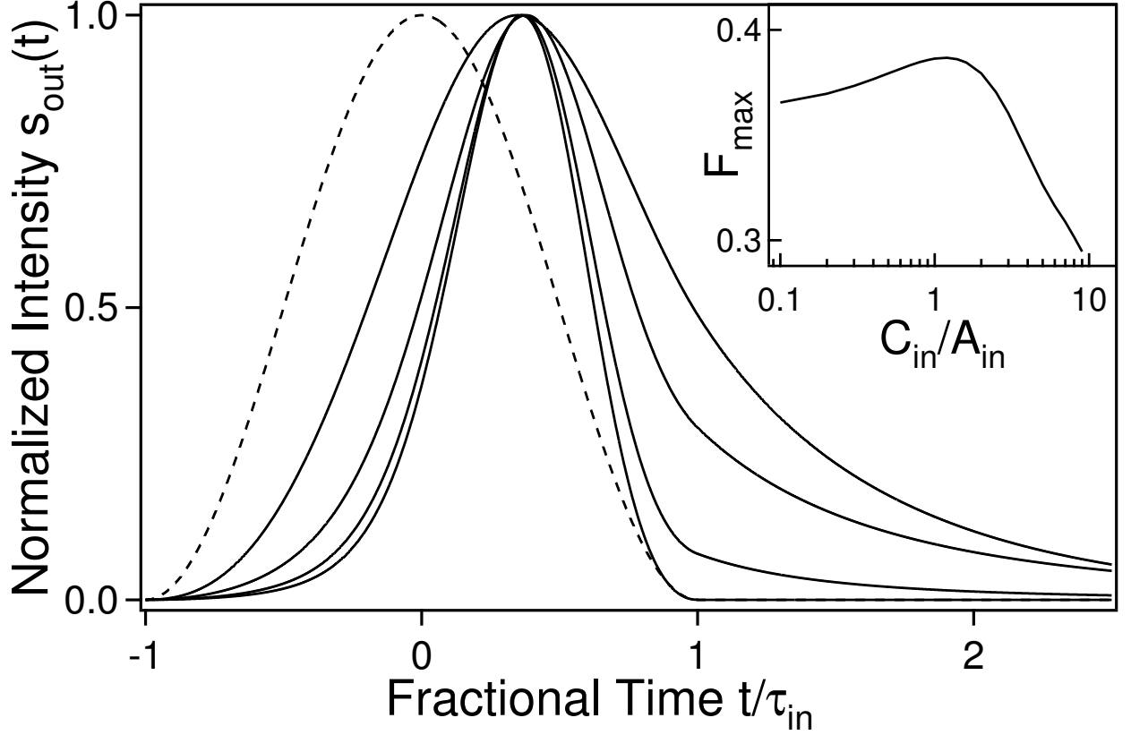
Figure 6: Intensity profile of the output pulses obtained for an overall peak intensity A_{in} + C_{in} = 10 . In order of increasing width, the represented profiles correspond to C_{in}/A_{in} = 0, 0.11, 0.54 and 9.0 . For each value of C_{in}/A_{in} , \tau/\tau_{in} is optimized in order to maximize the fractional delay. The profile of the input pulse (cos-pulse) is given for reference (dashed line). Inset: F_{max} as a function of C_{in}/A_{in} .
