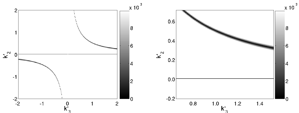
FIG. 2: Left panel : |a_2(k'_2, k'_3)| for gravity-capillary waves; Right panel : Close up showing the exact resonance near k'_2 = 0 . All variables are dimensionless, for notation and normalization see the text.
