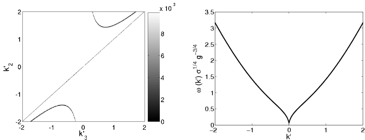
FIG. 1: Left panel : |a_1(k'_2, k'_3)| for gravity-capillary waves; Right panel: Corresponding dispersion relation \omega_{k'} . All variables are dimensionless, for notation and normalization see the text.
