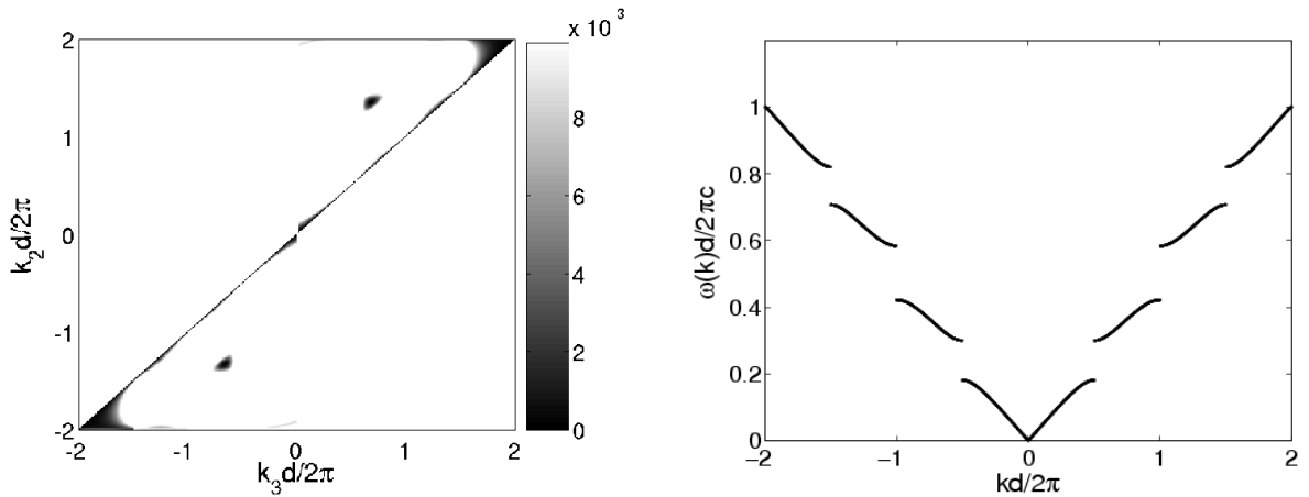
FIG. 3: Left panel : |a_1(k_2, k_3)| for a PC with refractive index contrast \Delta n = 2 ; Right panel: Corresponding photonic band structure \omega_k in the extended zone scheme.
