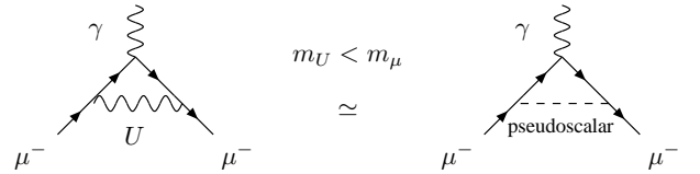
FIG. 4: For a light U as compared to m_\mu , the axial U -current contribution to g_\mu - 2 becomes equivalent to the one due to the exchange of a quasimassless pseudoscalar a , with axionlike couplings (cf. Sections II and V).
