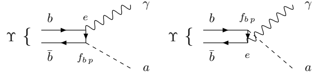
FIG. 6: When the U is light as compared to the \Upsilon , the sum of the decay amplitudes for \Upsilon \rightarrow \gamma U (Fig. 5) is essentially the same as for the production of a spin-0 pseudoscalar a in \Upsilon \rightarrow \gamma a , with a pseudoscalar a coupling to the b quark f_{bP} = f_{bA} \frac{2m_b}{m_U} = 2^{1/4} G_F^{1/2} m_b \frac{x}{x} = 2^{1/4} G_F^{1/2} m_b \cos \zeta \tan \beta [1, 5, 10].
