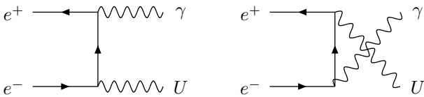
FIG. 2: Direct production of a U boson in e^+e^- annihilation. The U should decay preferentially into LDM particles if m_U > 2m_\chi , and otherwise into e^+e^- or possibly \nu\bar{\nu} pairs.
