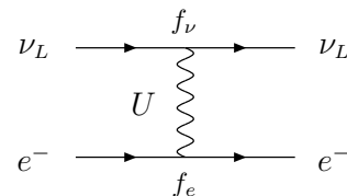
FIG. 8: U -exchange amplitude, contributing to low-energy \nu - electron scattering.
