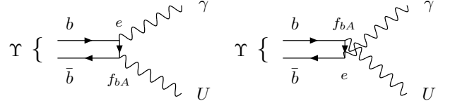
FIG. 5: Upsilon decay \Upsilon \rightarrow \gamma U , induced by the axial coupling f_{bA} of the U boson to the b quark. See also Fig. 6.
