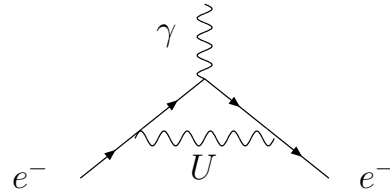
FIG. 3: U -exchange contribution to g_e - 2 .
