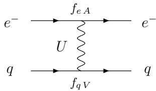
FIG. 7: U -exchange amplitude contributing to parity-violation effects in atomic physics [6, 7, 8].
