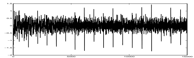
Figure 5: fECG obtained after wavelet baseline removal stage.
