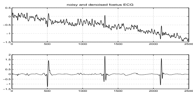
Figure 6: fECG obtained after baseline removal, PQRST amplification and wavelet de-noising stages.
