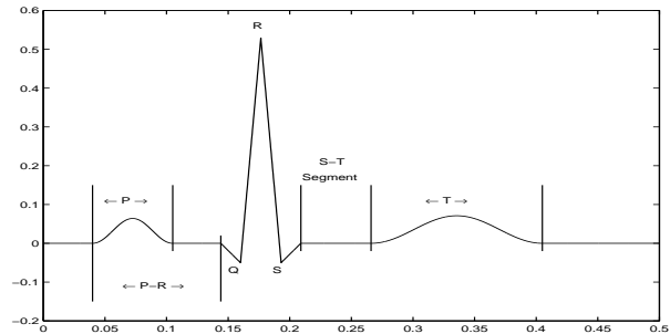
Figure 1: Decomposition of the ECG waveform.
