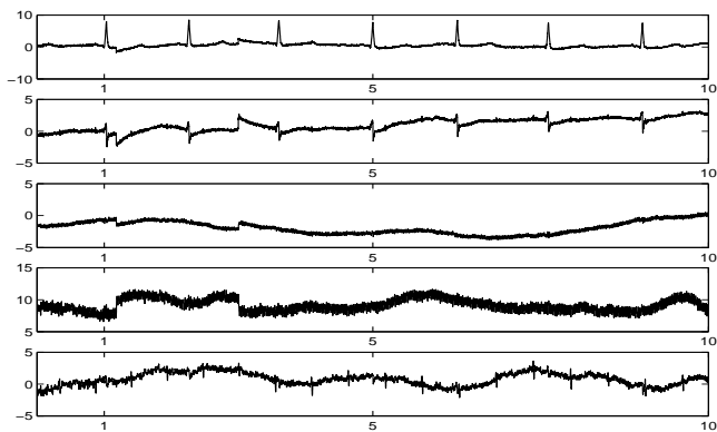
Figure 3: Estimated (separated) noisy source estimates with JADE algorithm.
