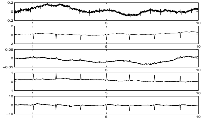
Figure 4: Estimated (separated) noisy source estimates with NS-joint diagonalization algorithm.
