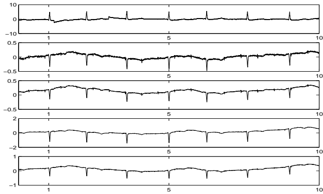
Figure 2: Five channels mother abdominal recording.
