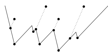
Figure 4: The projection of points onto flattened lower envelope.
