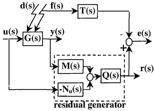
Fig 1. Scheme of robust residual generation.
