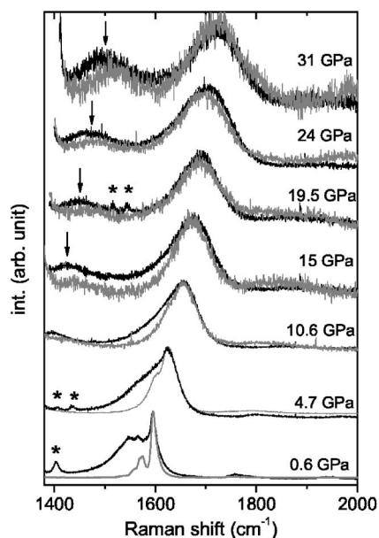
FIG. 3. Tangential modes Raman spectra as a function of pressure for both laser excitations: 514.5 nm in gray and 632.8 nm in black (experiment A). All the spectra are normalized. The stars indicate the presence of the ruby fluorescence. The peak visible at 1400\text{ cm}^{-1} at the higher pressures comes from the stressed diamond of the diamond anvil cell. The new band for pressures higher than 15 GPa is pointed out.
