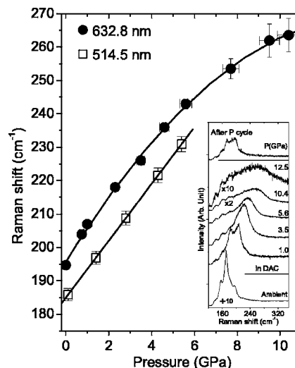
FIG. 2. Pressure dependence of the most intense component of the radial breathing modes (RBM) of SWNT for a laser excitation of 514.5 nm (squares) and 632.8 nm (circles) up to the signal disappearance (experiment A). The right inset shows the spectra of the RBM at different pressures for a laser excitation of 632.8 nm. The two ambient pressure spectra were taken outside the diamond anvil cell.
