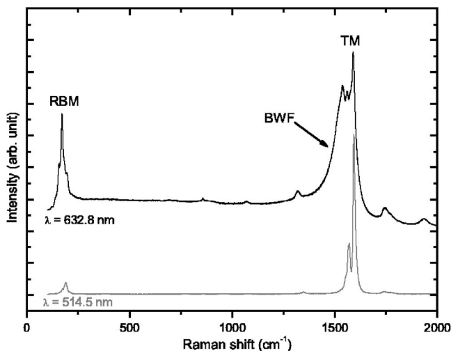
FIG. 1. Raman spectra of SWNT at ambient pressure recorded using two different laser excitation (632.8 nm top and 514.5 nm bottom). The Breit Wigner Fano component (BWF) is pointed out. No pressure transmitting medium was used to record those spectra.
