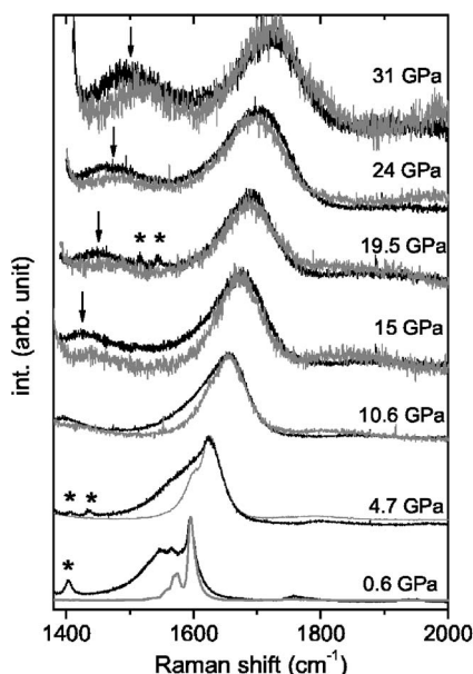
FIG. 3. Tangential modes Raman spectra as a function of pressure for both laser excitation: 514.5 nm in gray and 632.8 nm in black (experiment A). All the spectra are normalized. The stars indicate the presence of the ruby fluorescence. The peak visible at 1400 cm -1 at the higher pressures comes from the stressed diamond of the diamond anvil cell. The new band for pressures higher than 15 GPa is pointed out.
