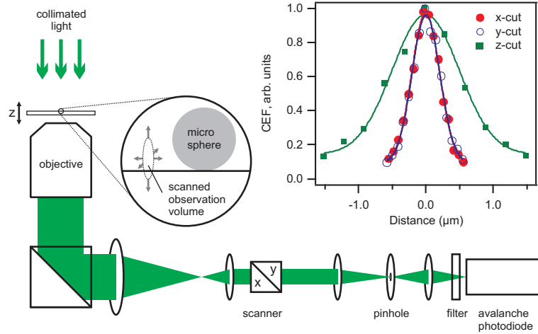
FIG. 1: Schematic of the observation setup (not to scale). The observation volume can be scanned in 3D by acting on both scanner and focus. Inset: Measured CEF for the system.
