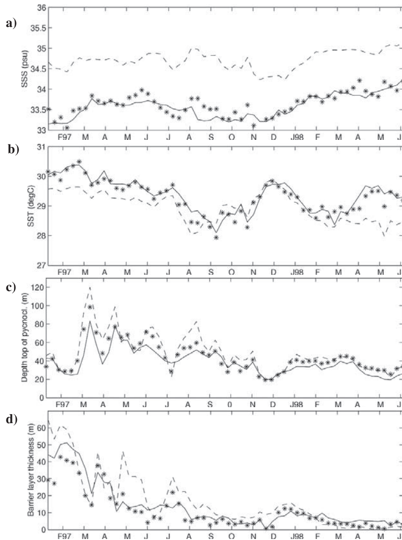
Figure 13. Time evolution of (a) SSS, (b) SST, (c) depth of top of pycnocline, and (d) barrier layer thickness at ( 0^{\circ}\text{N} , 155^{\circ}\text{E} ) for REF (continuous line), FREE (dashed line), and ASSIM (stars).
