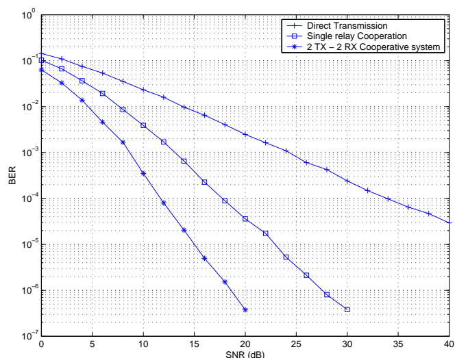
Fig. 3. uncoded multi-branch cooperative transmission
