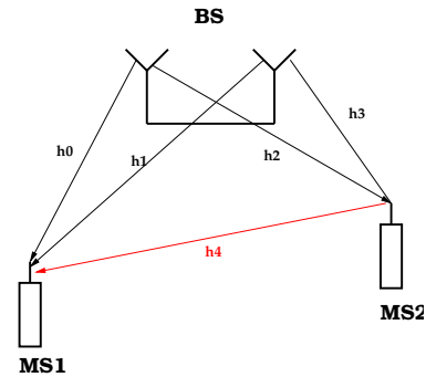
Fig. 1. 2 BS antennas and 1 relaying MS emulating the (2,2) Alamouti scheme
