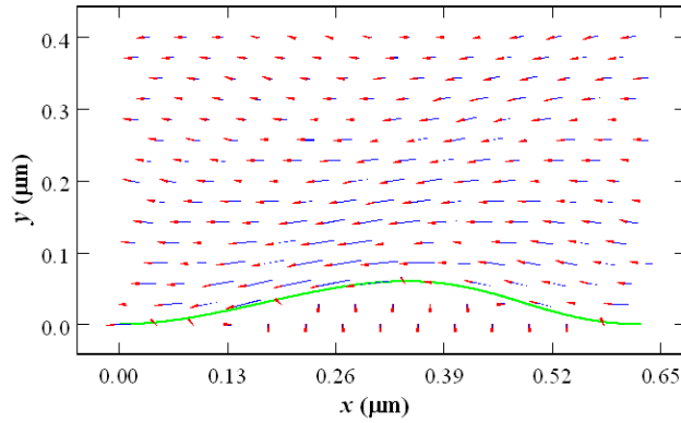
Fig. 6. Poynting vectors plotted in the near field area above a sinusoidal grating illuminated in normal incidence. d = 626.67 nm, \alpha = 27.5^\circ and h = 59.94 nm.
