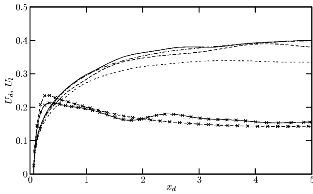
FIG. 9. Nondimensional velocities of the dense and light fronts, respectively, U_d and U_l as functions of the nondimensional dense front position x_d for \alpha=20.6 and Re=\rho_{\text{air}}h\sqrt{\alpha gh}/\mu_{\text{air}} . Velocity U_d (upper curves): ---, no-slip boundary condition and \lambda=1+\alpha\Phi (constant kinematic viscosity); -.-, no-slip condition and \lambda=1 (constant dynamic viscosity); —, free slip condition and \lambda=1+\alpha\Phi ; —, free slip condition and \lambda=1 . Velocity U_l (lower curves): - \times -, no-slip condition and \lambda=1 ; \times -, free slip condition and \lambda=1 .
