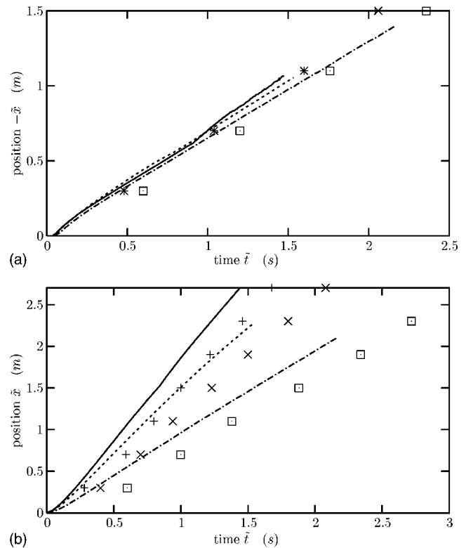
FIG. 5. Comparison of the numerical and experimental results (in dimensional units). Plot (a) light front, plot (b) dense front. —, Numerical results for \alpha=20.6 and + , experimental values. ---, Numerical results for \alpha=8.93 and \times , experimental values. -.-, Numerical results for \alpha=1.99 and \square , experimental values. The Reynolds number in the simulations is the same as in the experiments.
