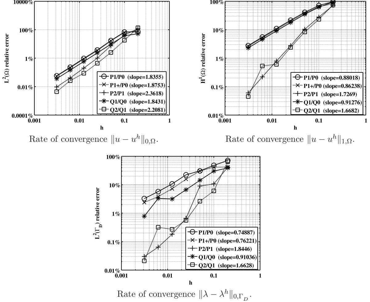
Figure 15: Rates of convergence for some couples of finite element spaces with the fully stabilized method.
