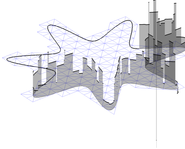
Figure 13: Multiplier on \Gamma_D with the Barbosa-Hughes stabilization for the P_1/P_0 method ( h = 0.05 ).
