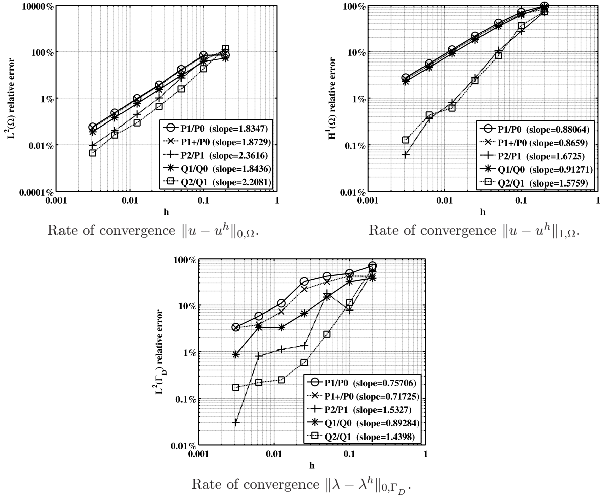
Figure 12: Rates of convergence for some couples of finite element spaces with the Barbosa-Hughes stabilization.
