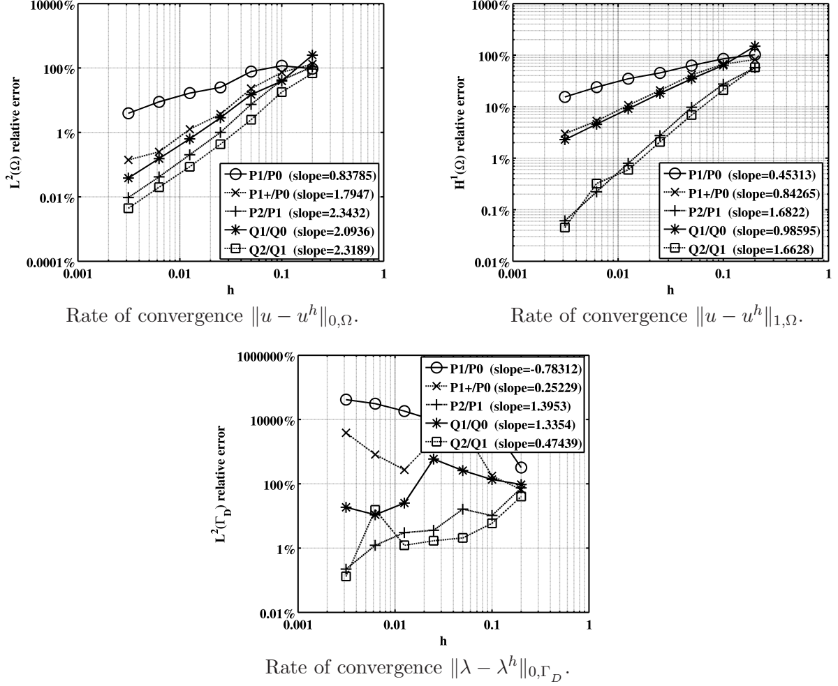
Figure 8: Rates of convergence for some couples of finite element spaces with no stabilization.
