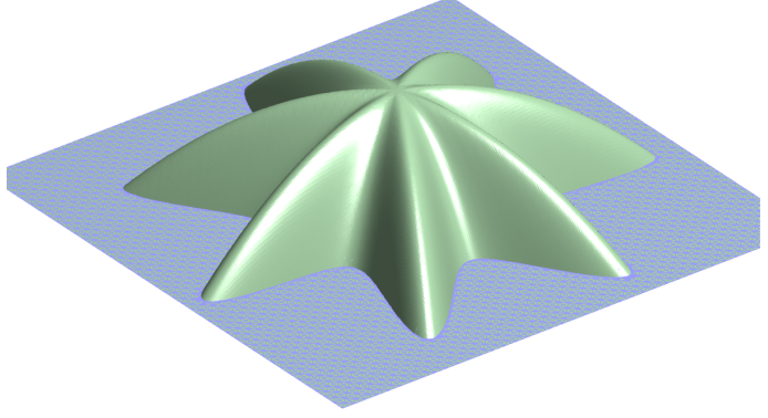
Figure 6: Exact solution.
