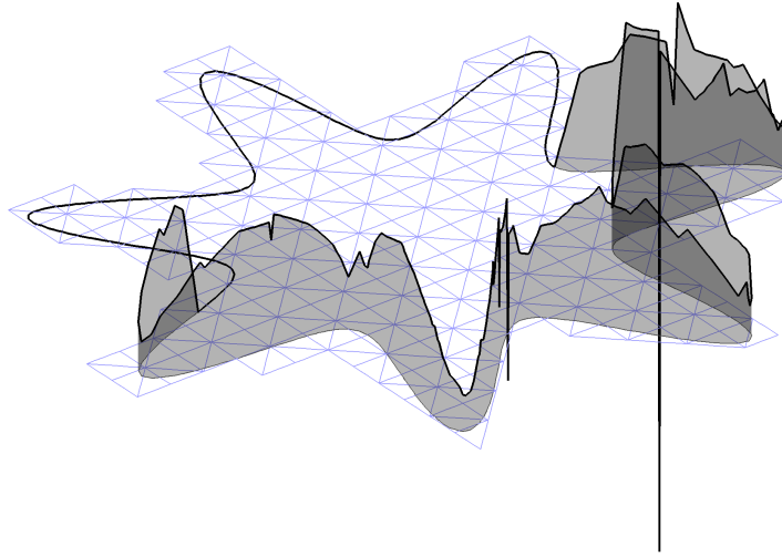
Figure 11: Multiplier on \Gamma_D with no stabilization for the P_2/P_1 method ( h = 0.05 ).
