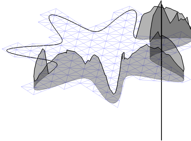
Figure 14: Multiplier on \Gamma_D with the Barbosa-Hughes stabilization for the P_2/P_1 method ( h = 0.05 ).
