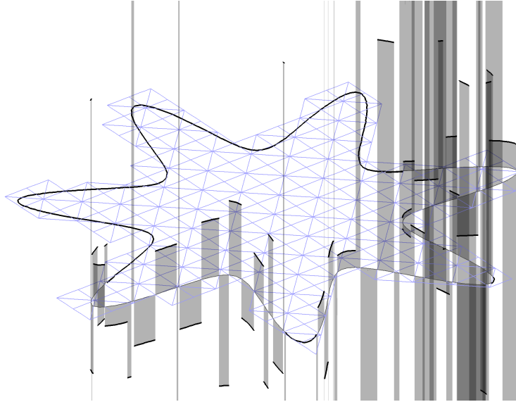
Figure 10: Multiplier on \Gamma_D with no stabilization for the P_1/P_0 method ( h = 0.05 ).
