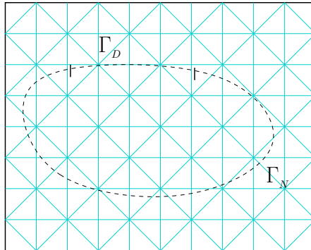
Figure 2: Example of a structured mesh.
