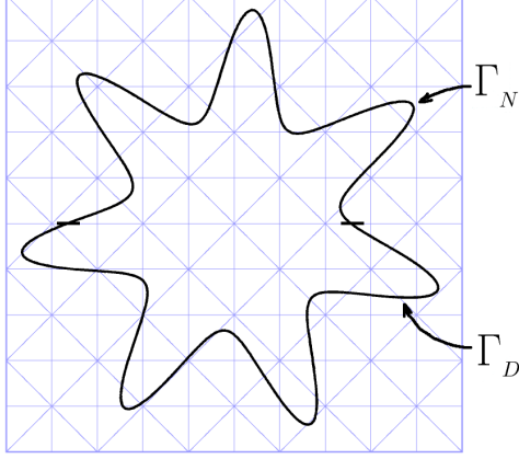
Figure 5: Test domain and a triangular structured mesh.
