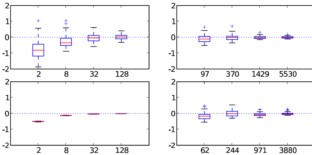
638 639 640 641 642 643 644 645 646 647 648 649 650 651 652 653 654 655 656 657 658 659 660 661 662 663 Fig. 5. Probit example: Box-plots of ( left column ) log- errors of nested importance sampling estimates, for N = 2, 8, 32, 128, compared with the log-error of importance sampling estimates ( right column ) based on the optimal Gaussian proposal, and the same number of likelihood evaluation (reported on the x axis of the right column plots). Bottom row corresponds to the first strategy (both mode and Hessian available), top row corresponds to the second strategy (only mode available).
