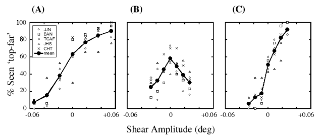
Fig. 11: Rate of 'top-far' perception with respect to the strength of the stimulus (Naji and Freeman 2004). Condition A corresponds to a translating object without eye pursuit; condition B to a rotating object and condition C to a translating object with pursuit. Conditions A and B show that translation allows for a disambiguation, contrary to passive rotation. Furthermore, the comparison of conditions A and C shows that pursuit of the object leads to better perception.
