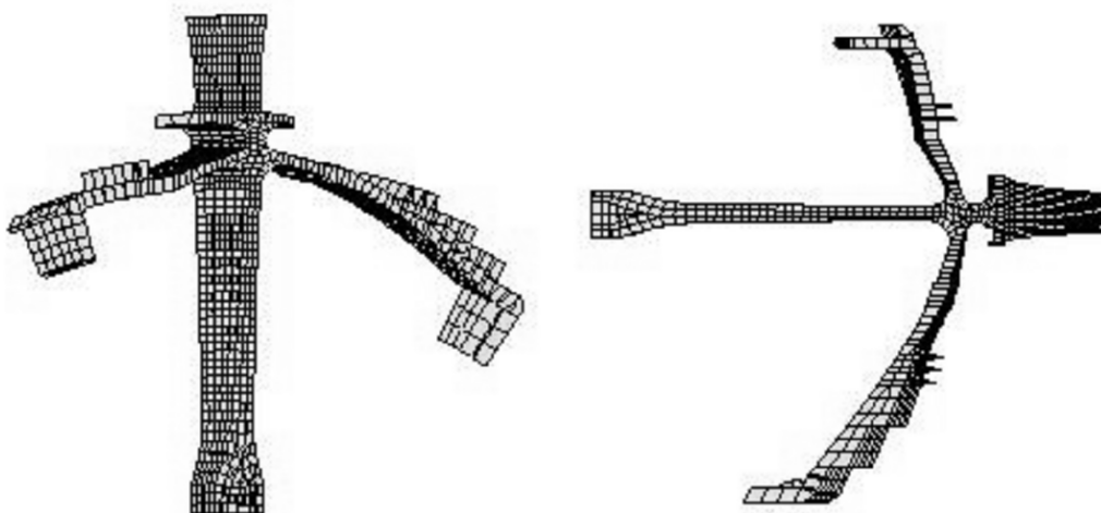
Figure 2: finite element model of a blisk sector
