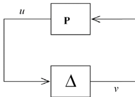
Figure 1 : \mathbf{P} - \Delta feedback connection
