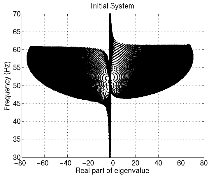
Figure 15 : Frequency and real part of eigenvalue of the initial system for various friction coefficient \mu_f and stiffness k_1
