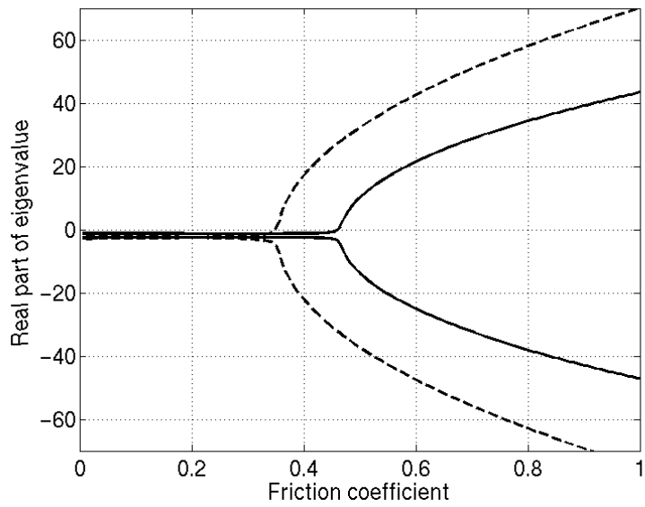
Figure 8 : Evolution of the real part of two coupling modes (----- Initial system, ——— Controlled system)
