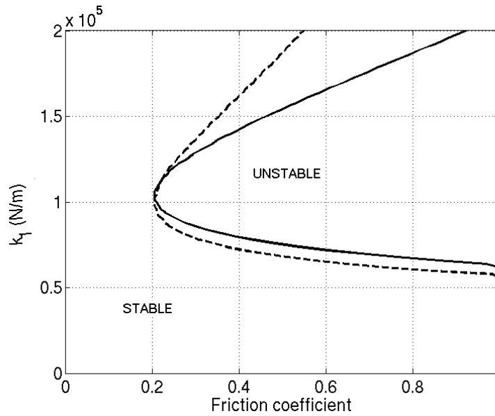
Figure 10 : Stability as a function of brake friction coefficient \mu_f and stiffness k_1 (----- Initial system, ——— Controlled system)
