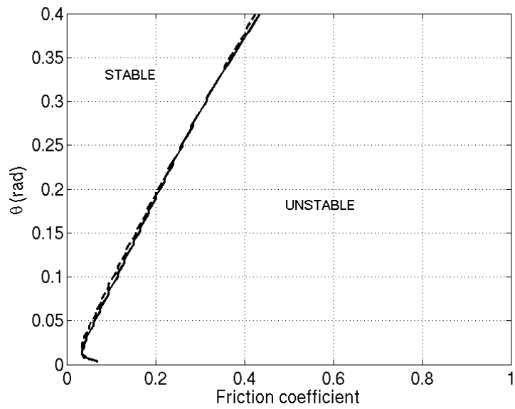
Figure 14 : Stability as a function of brake friction coefficient \mu_f and angle \theta (----- Initial system, ——— Controlled system)
