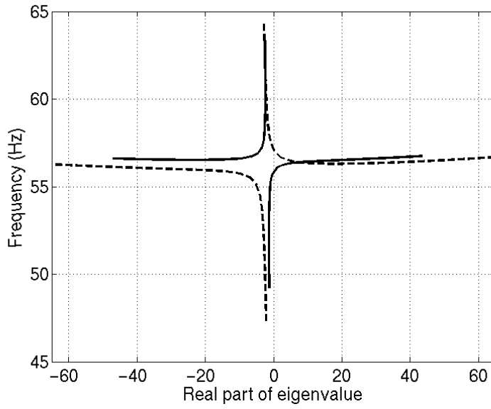
Figure 9 : Evolution of the frequency versus real part of two coupling modes (----- Initial system, ——— Controlled system)
