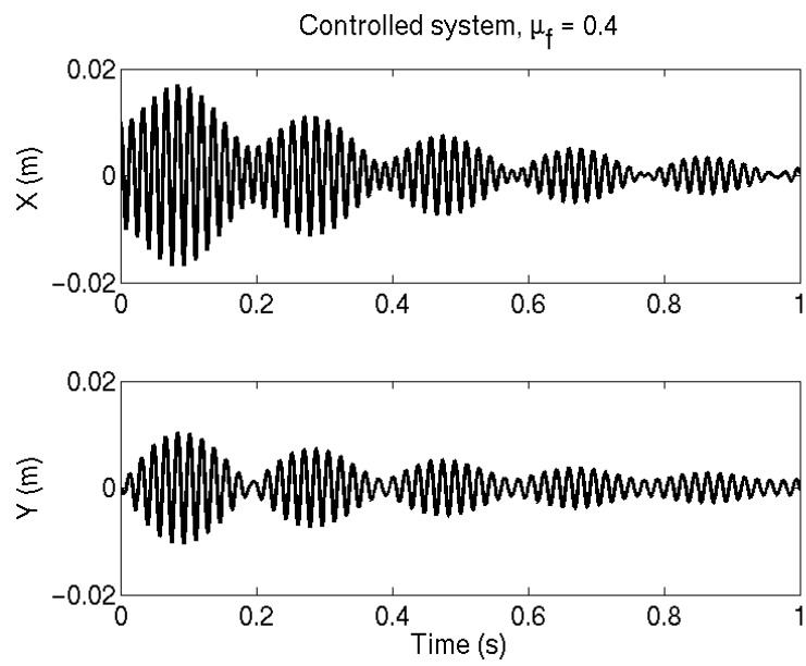
Figure 18 : Temporal response of the controlled system for \mu_f = 0.4
