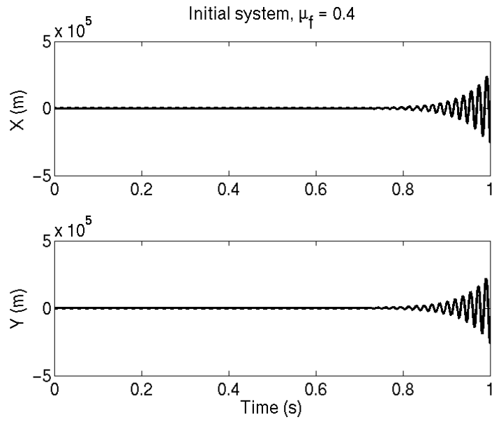
Figure 17 : Temporal response of the initial system for \mu_f = 0.4
