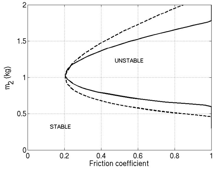
Figure 13 : Stability as a function of brake friction coefficient \mu_f and mass m_2 (----- Initial system, ——— Controlled system)
