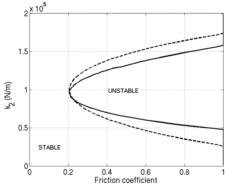
Figure 11 : Stability as a function of brake friction coefficient \mu_f and stiffness k_2 (----- Initial system, ——— Controlled system)
