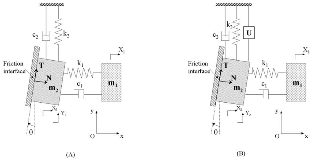
Figure 3 : Braking model (A) initial system (B) controlled system
