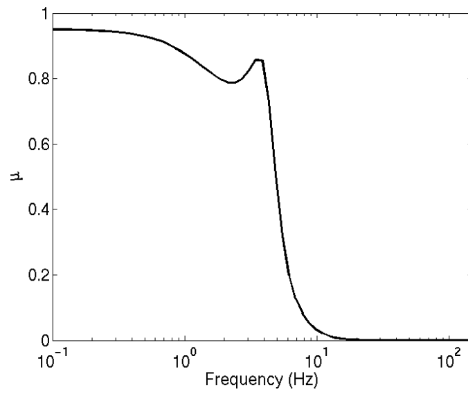
Figure 4 : Evolution of the structured singular value \mu
