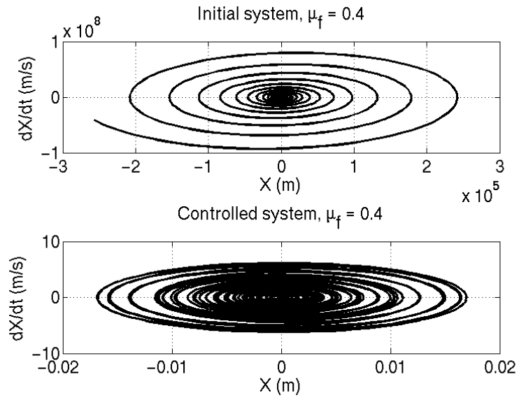
Figure 19 : Divergent oscillations for \mu_f = 0.4 ( \mu_{f0} < \mu_f < \tilde{\mu}_{f0} )
