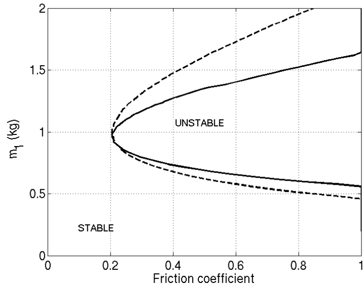
Figure 12 : Stability as a function of brake friction coefficient \mu_f and mass m_1 (----- Initial system, ——— Controlled system)
