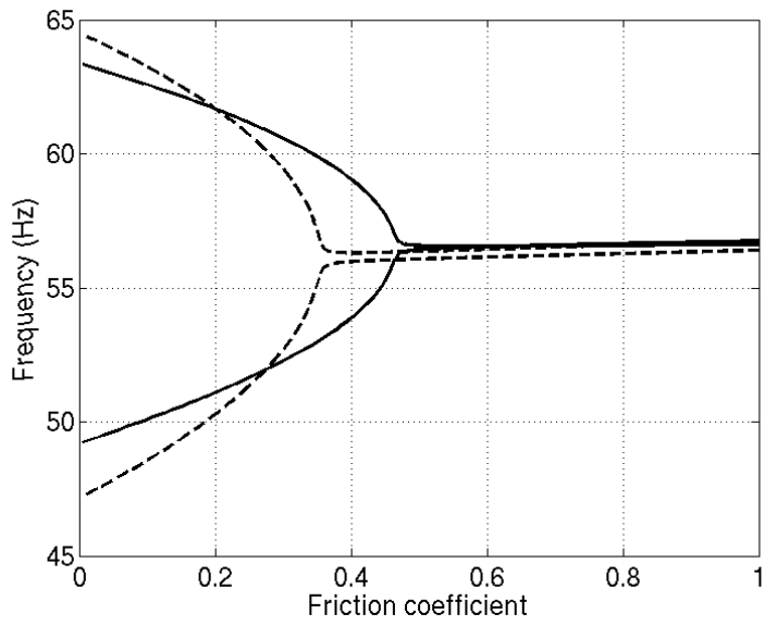
Figure 7 : Evolution of the frequency of two coupling modes (----- Initial system, ——— Controlled system)
