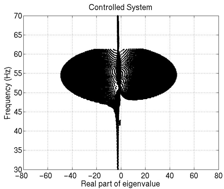
Figure 16 : Frequency and real part of eigenvalue of the controlled system for various friction coefficient \mu_f and stiffness k_1
