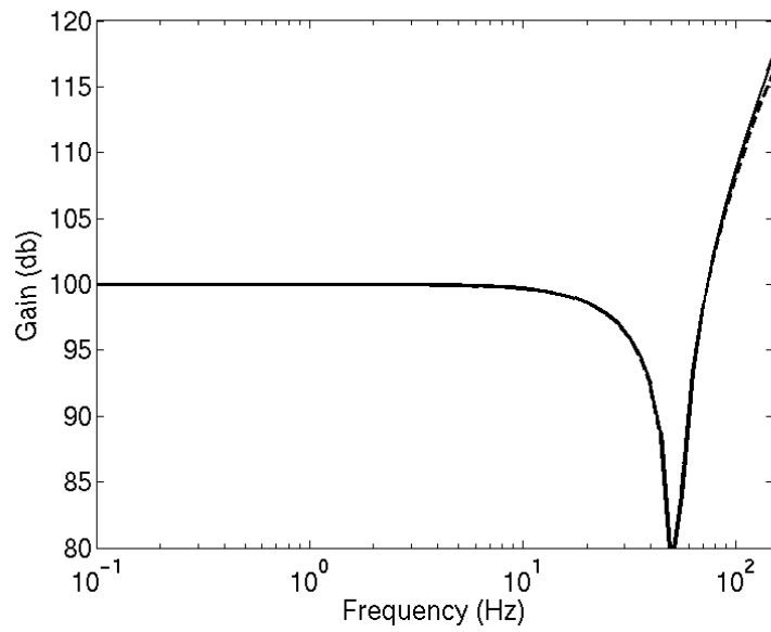
Figure 6 : Approximation of the controller (----- Result of the \mu -synthesis, ——— Approximation)
