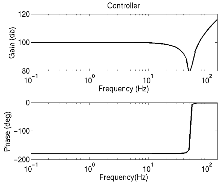
Figure 5 : Bode diagram of the controller
