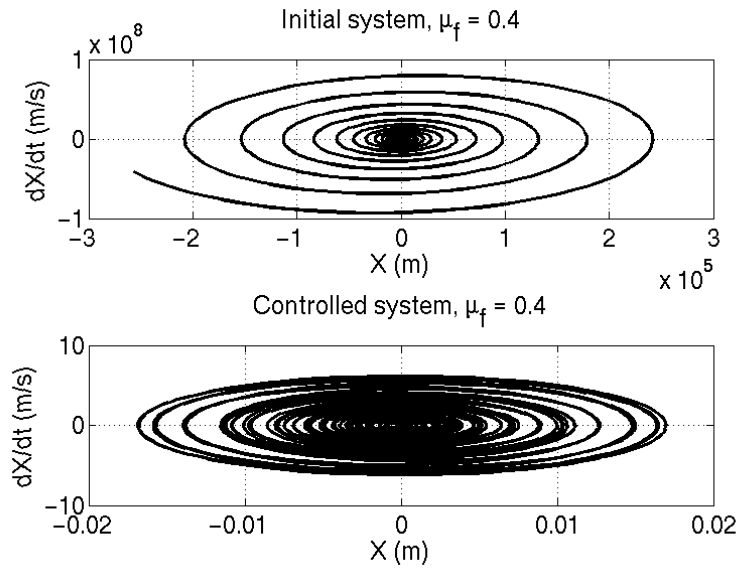
Figure 19 : Divergent oscillations for \mu_f = 0.4 ( \mu_{f0} < \mu_f < \tilde{\mu}_{f0} )
