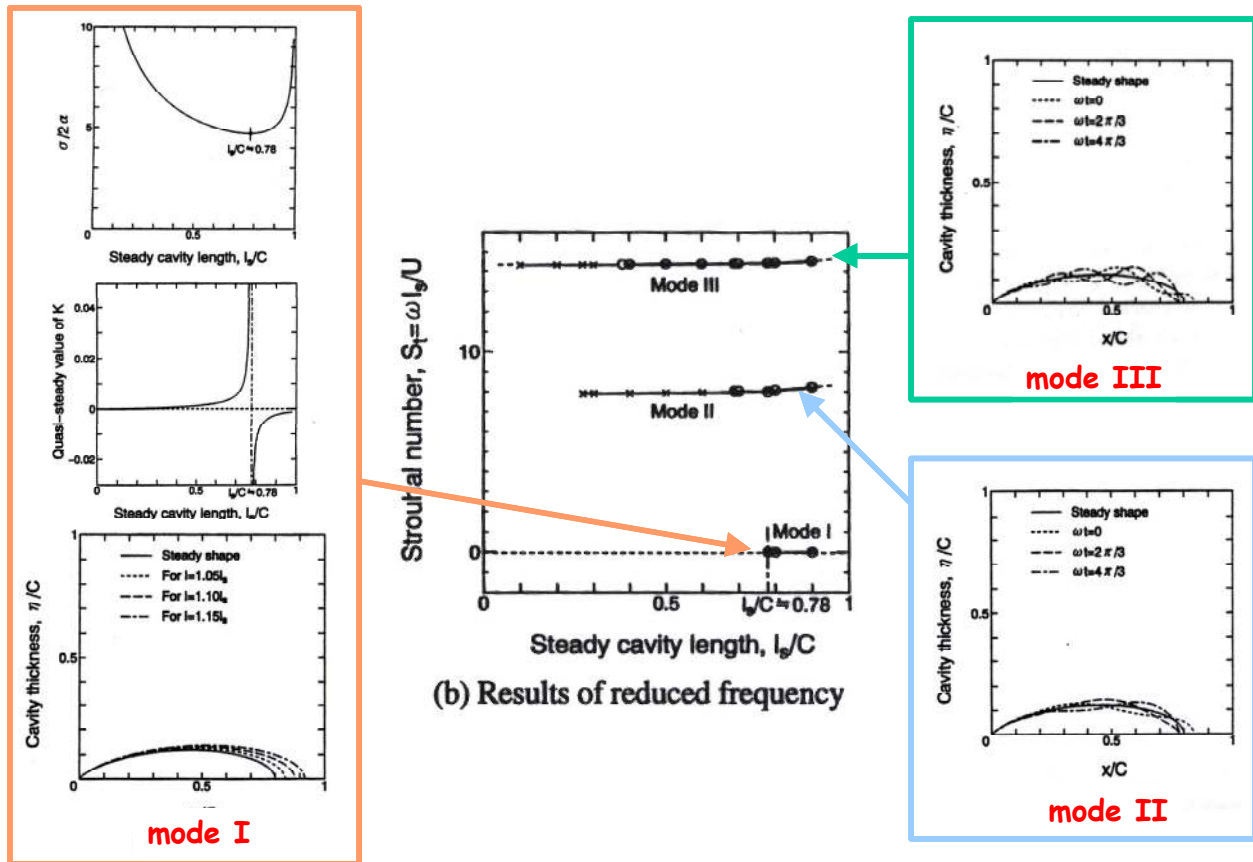
Figure 24: Various modes of instability deduced from a linear analysis of the stability of two-dimensional partial cavities. The central part of the figure gives the Strouhal number of modes I, II and III. The evolution in time of the cavity interface is also indicated for each mode (reproduced from Watanabe et al. 1998).
