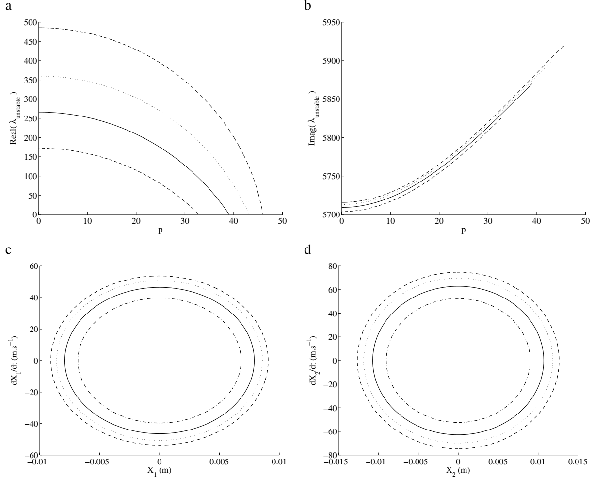
Figure 6: Evolutions of the unstable mode and the associated limit cycles for \mu = 0.3 and k^{NL} = 10^{11} N.m^{-3} with proportional structural damping ( -- c_1 = c_2 = 125.7 N.m^{-1} s^{-1} , \cdots c_1 = c_2 = 377 N.m^{-1} s^{-1} , - c_1 = c_2 = 565.5 N.m^{-1} s^{-1} , -.- c_1 = c_2 = 754 N.m^{-1} s^{-1} ) (a) real parts (b) associated imaginary part (c) limit cycles (X_1, \dot{X}_1) (d) limit cycles (X_2, \dot{X}_2)
