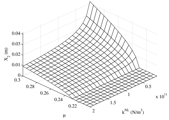
Figure 13: Amplitudes of the displacements X_1 and X_2 as a function of the friction coefficient \mu and the cubic non-linearity k^{\text{NL}} (with \eta_1 = \eta_2 = 0.06 ) (a) initial real part for p = 0 (b) final frequency (c) \text{Max}(X_1) (d) \text{Max}(X_2)
