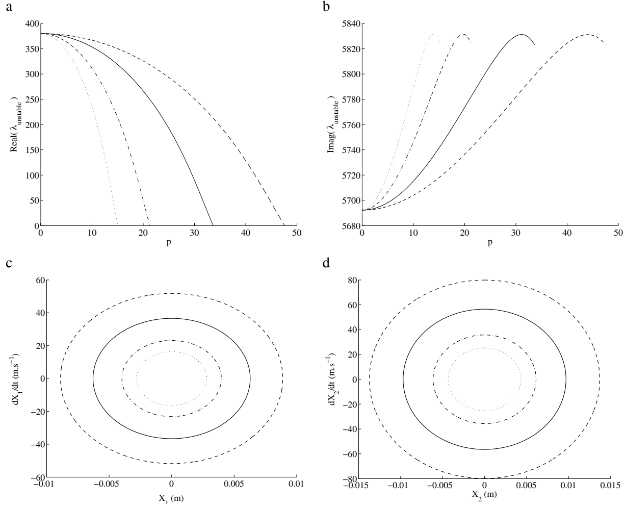
Figure 10: Evolutions of the unstable mode and the associated limit cycles for \mu = 0.3 and \eta = \eta_2 = 0.06 (... k^{NL} = 10^{11} N.m^{-3} , -.- k^{NL} = 5.10^{10} N.m^{-3} , - k^{NL} = 2.10^{10} N.m^{-3} , - - k^{NL} = 10^{10} N.m^{-3} ) (a) real parts (b) associated imaginary part (c) limit cycles (X_1, \dot{X}_1) (d) limit cycles (X_2, \dot{X}_2)
