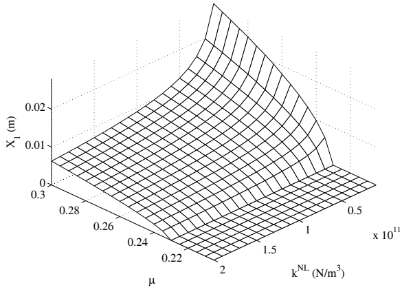
Figure 13: Amplitudes of the displacements X_1 and X_2 as a function of the friction coefficient \mu and the cubic non-linearity k^{\text{NL}} (with \eta_1 = \eta_2 = 0.06 ) (a) initial real part for p = 0 (b) final frequency (c) \text{Max}(X_1) (d) \text{Max}(X_2)
