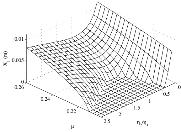
Figure 12: Amplitudes of the displacements X_1 and X_2 as a function of the friction coefficient \mu and the damping ratio \frac{\eta_2}{\eta_1} (with \eta_1 = 0.06 and k^{NL} = 10^{11} \text{ N.m}^{-3} ) (a) initial real part for p = 0 (b) final frequency (c) Max(X_1) (d) Max(X_2)
