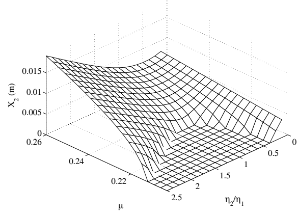
Figure 12: Amplitudes of the displacements X_1 and X_2 as a function of the friction coefficient \mu and the damping ratio \frac{\eta_2}{\eta_1} (with \eta_1 = 0.06 and k^{NL} = 10^{11} \text{ N.m}^{-3} ) (a) initial real part for p = 0 (b) final frequency (c) Max(X_1) (d) Max(X_2)
