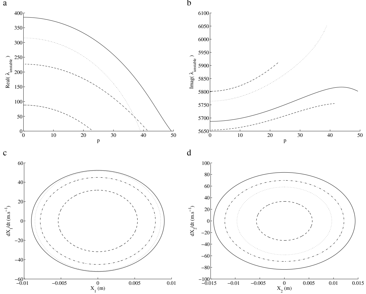
Figure 8: Evolutions of the unstable mode and the associated limit cycles for \mu = 0.3 and k^{NL} = 10^{11} N.m^{-3} with non-proportional structural damping (— c_1 = 754 Nm^{-1}s^{-1} and c_2 = 301.6 Nm^{-1}s^{-1} , \cdots c_1 = 377 Nm^{-1}s^{-1} and c_2 = 603.2 Nm^{-1}s^{-1} , - c_1 = 502.7 Nm^{-1}s^{-1} and c_2 = 201.1 Nm^{-1}s^{-1} , - . - c_1 = 251.3 Nm^{-1}s^{-1} and c_2 = 402.1 Nm^{-1}s^{-1} ) (a) real parts (b) associated imaginary part (c) limit cycles (X_1, \dot{X}_1) (d) limit cycles (X_2, \dot{X}_2)
