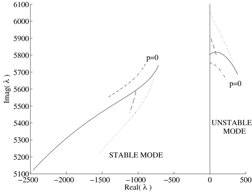
Figure 9: Evolution of the stable and unstable modes in the complex plane with non-proportional structural damping ( - - c_1 = 754Nm^{-1}s^{-1} and c_2 = 1131Nm^{-1}s^{-1} , \dots c_1 = 377Nm^{-1}s^{-1} and c_2 = 565.5Nm^{-1}s^{-1} , - c_1 = 377Nm^{-1}s^{-1} and c_2 = 282.75Nm^{-1}s^{-1} , - . - c_1 = 754Nm^{-1}s^{-1} and c_2 = 565.5Nm^{-1}s^{-1} )
