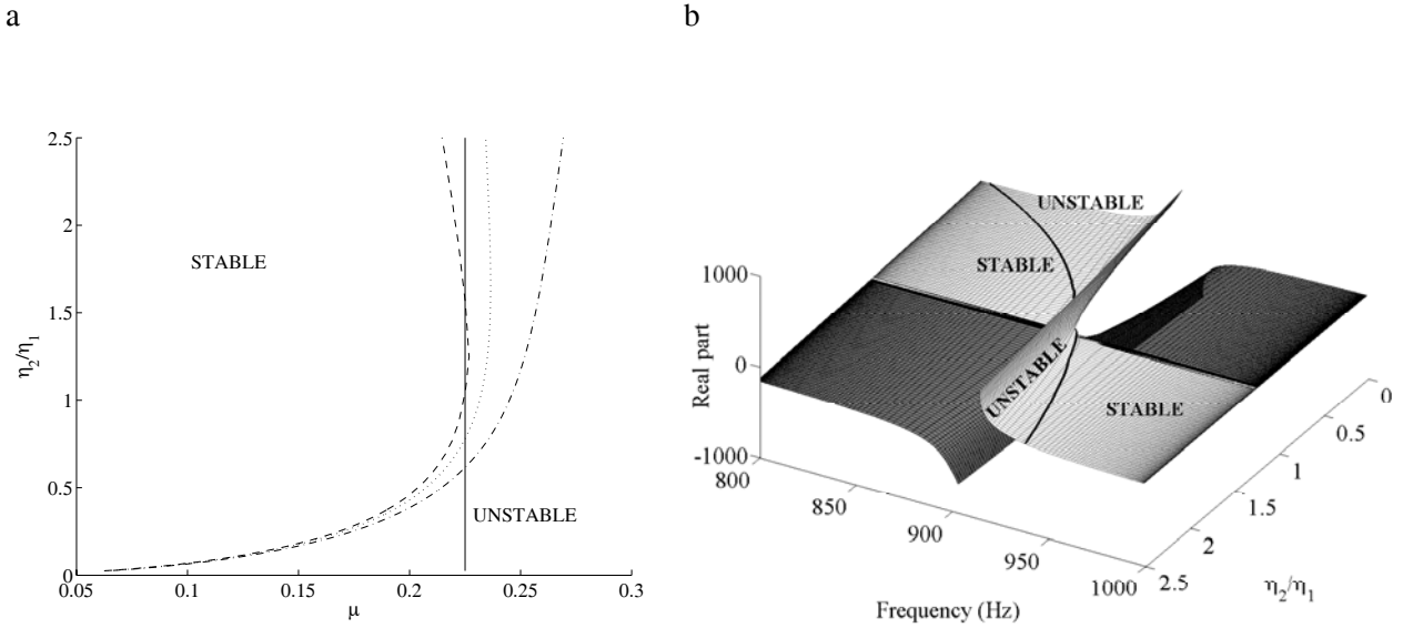
Figure 2: Effects of the damping on the stability (a) Stable and unstable zones versus the damping ratio \frac{\eta_2}{\eta_1} and the friction coefficient \mu (— undamped, — \eta_2 = 0.02 , \cdots \eta_2 = 0.06 , — \eta_2 = 0.1 ) (b) Evolution of the stable and unstable modes in the complex plane for \eta_2 = 0.02
