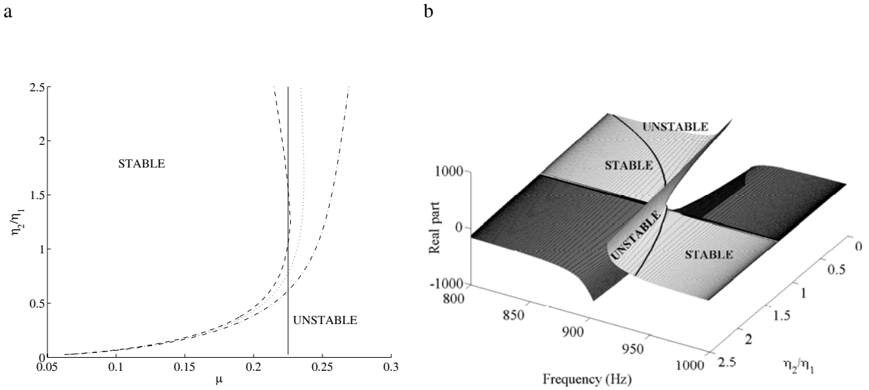
Figure 2: Effects of the damping on the stability (a) Stable and unstable zones versus the damping ratio \frac{\eta_2}{\eta_1} and the friction coefficient \mu (— undamped, — \eta_1 = 0.02 , \cdots \eta_1 = 0.06 , — \eta_1 = 0.1 ) (b) Evolution of the stable and unstable modes in the complex plane for \eta_h = 0.02
