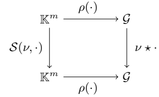
Figure 2: \mathcal{G} -equivariance of the moving frame \rho .
