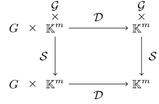
Figure 1: Diagram involving a dynamical system \mathcal{D} and one of its Lie symmetries \mathcal{S} .
