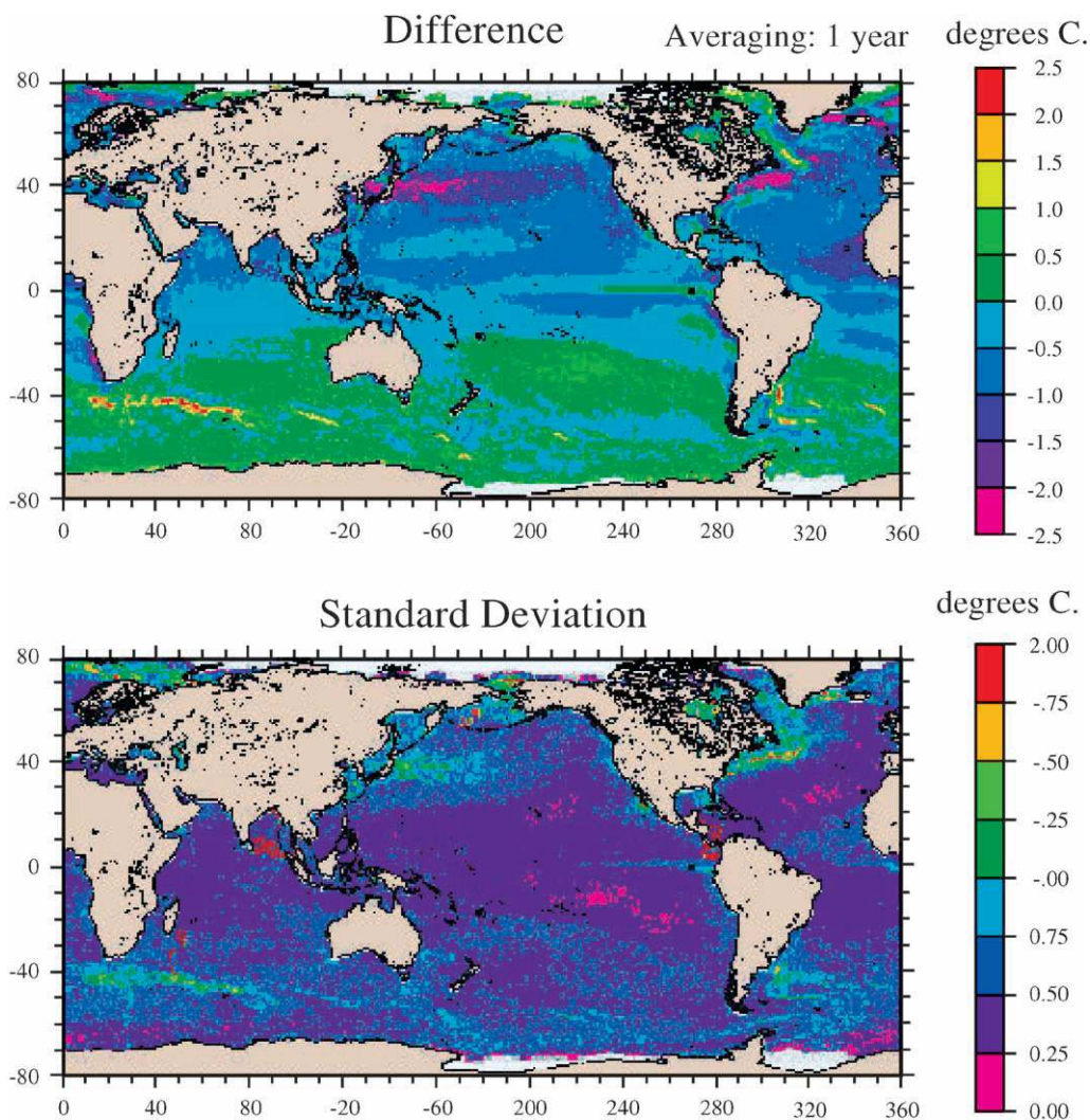
Fig. 2. Top panel: 1-year (1993) average of the differences between our SST product and Reynolds SST. Lower panel: 1-year standard deviation of the differences between our SST product and Reynolds SST.
