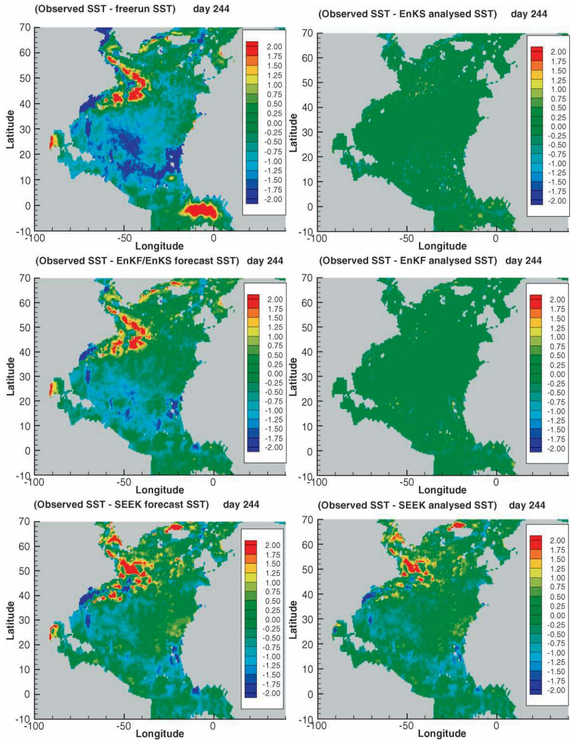
Fig. 9. Numerical results for SST field, day 244 1996.
