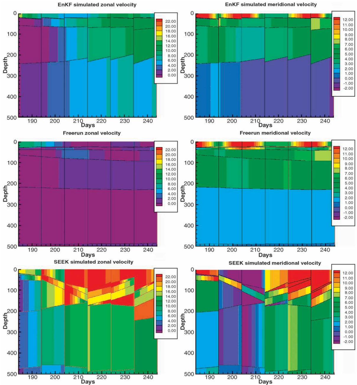
Fig. 17. Time–depth sections of observed and simulated zonal velocity (left) and meridional velocity (right). EnKF data (upper), free-run data (middle) and SEEK data (lower).
