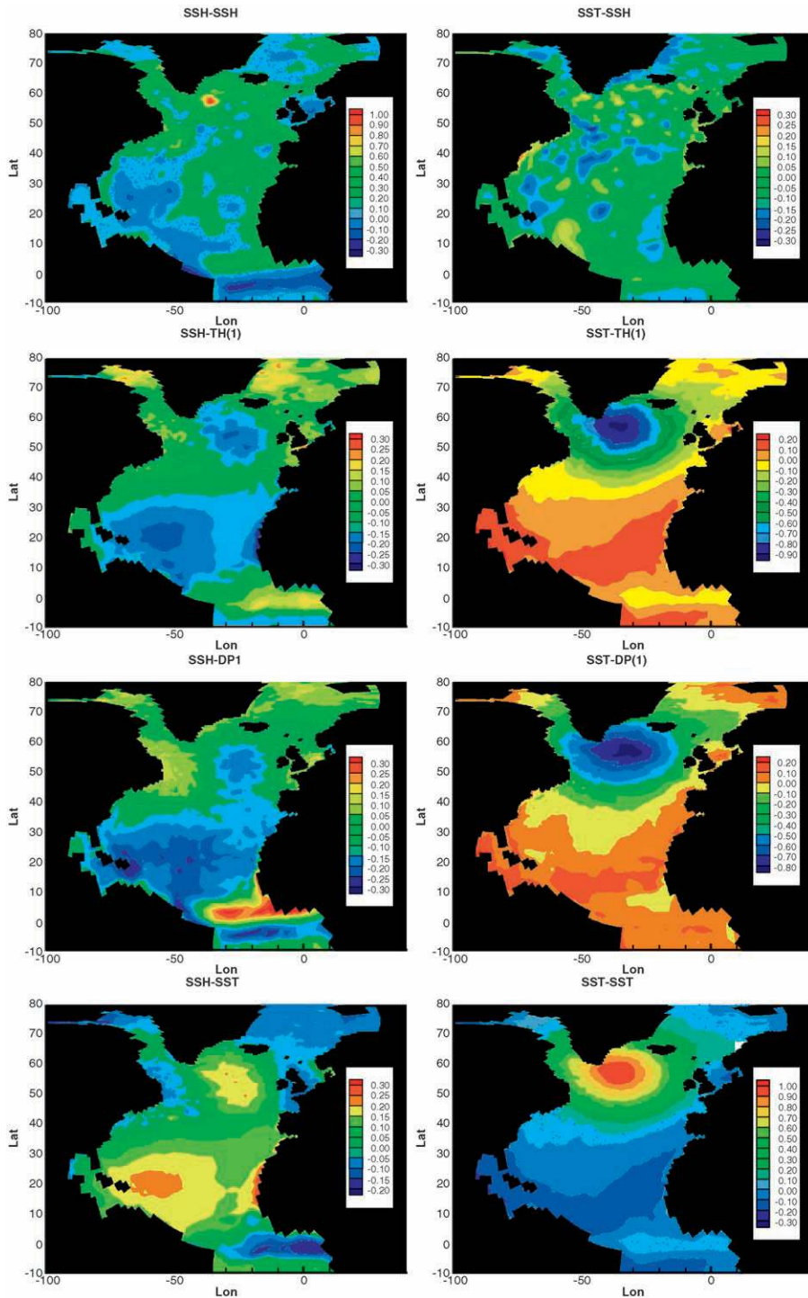
Fig. 5. Correlations between MICOM variables corresponding to location 37^{\circ}\text{W} and 57.5^{\circ}\text{N} , calculated from EnKF forecast ensemble day 184.
