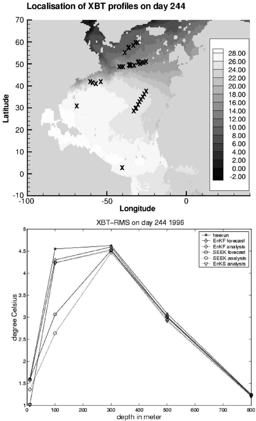
Fig. 19. The localisation of the XBT data on day 244 (upper) and the corresponding RMSE versus depth plot for the free-run, EnKF, EnKS and SEEK assimilation runs (lower).
