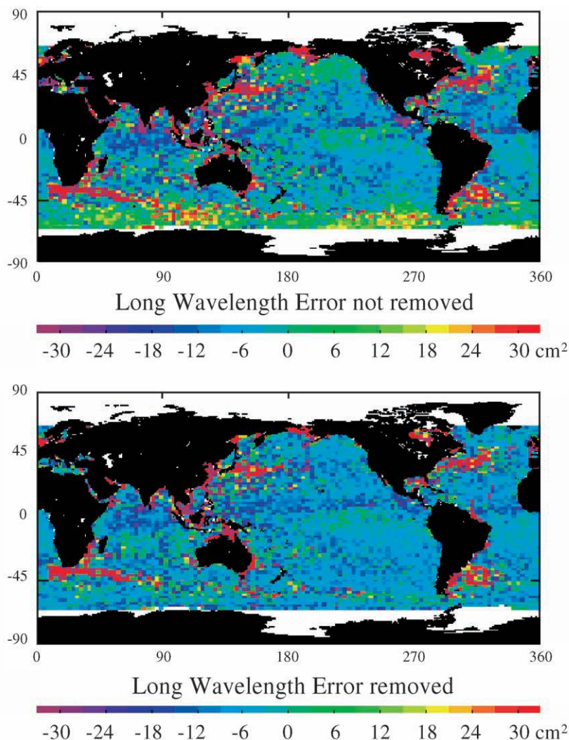
Fig. 1. The difference between the 1-year SLA variance (in cm 2 ) observed by T/P and ERS. Top panel: before Long Wavelength Errors (LWE) are removed, bottom panel: after LWE removal.
