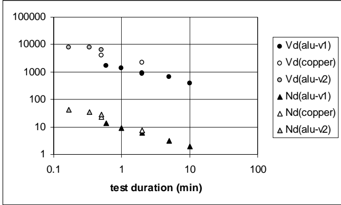
Figure 1: Volume damage rate V_d ( \mu\text{m}^3\text{mm}^{-2}\text{s}^{-1} ) and pit number rate N_d ( \times 10^2\text{pits.mm}^{-2}.\text{s}^{-1} ) as a function of test duration for copper ( v = 38.5 \text{ m.s}^{-1} ) and aluminum samples ( v_1 = 20 \text{ m.s}^{-1} & room temperature ; v_2 = 32 \text{ m.s}^{-1} & 30^\circ\text{C} ) [1]
